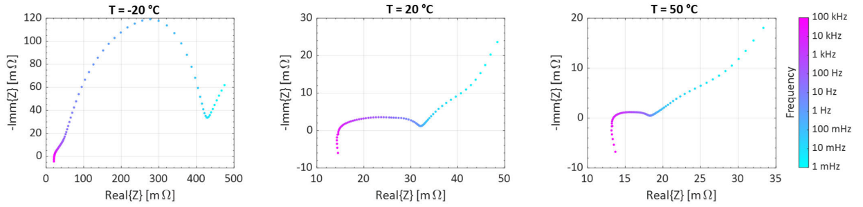
Fig. 6. Results of the impedance spectroscopy measurements performed at \text{SOC} = 40\% for three different temperatures (minimum value, standard conditions, and maximum value).
