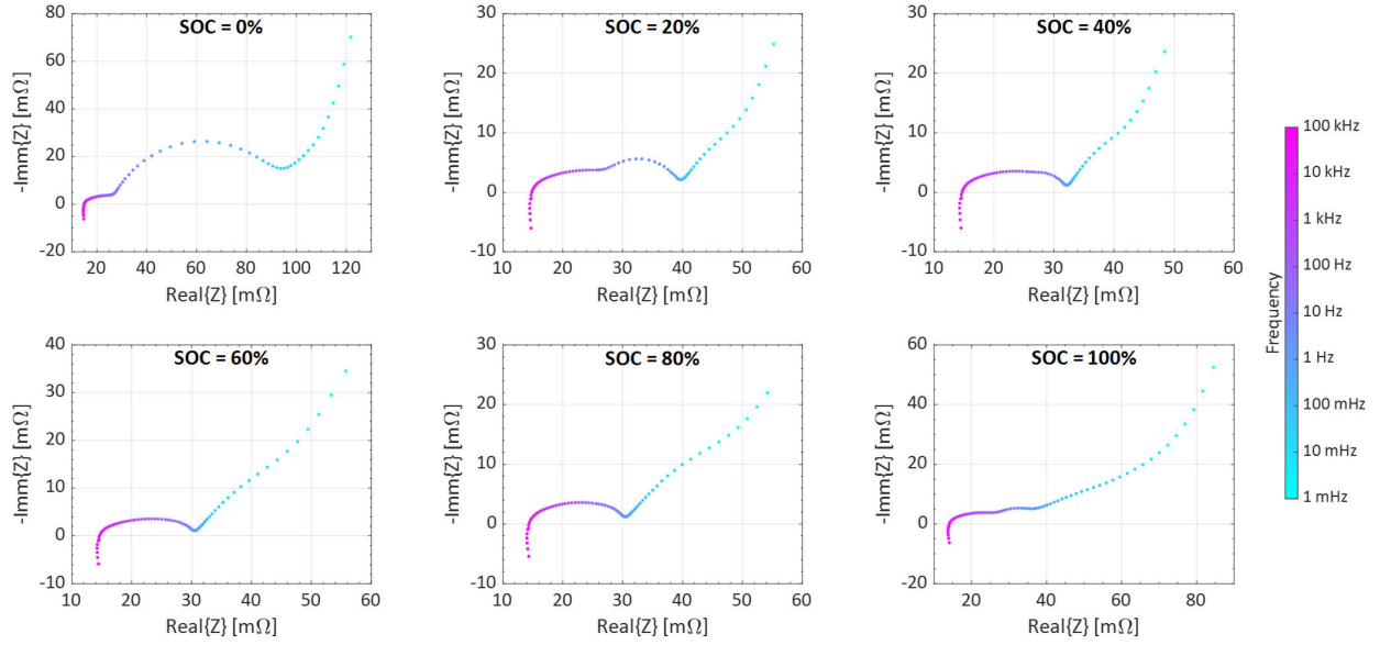
Fig. 5. Results of the impedance spectroscopy measurements at T = 20\text{ }^{\circ}\text{C} for all the different analyzed SOC levels. The colormap emphasizes the frequency of investigation.
