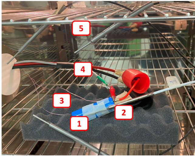
Fig. 3. Detail of the setup inside the climatic chamber showing—1: SC under test, 2: control PT100, 3: safety thermocouples, 4: electric connections; and 5: additional temperature sensors.
