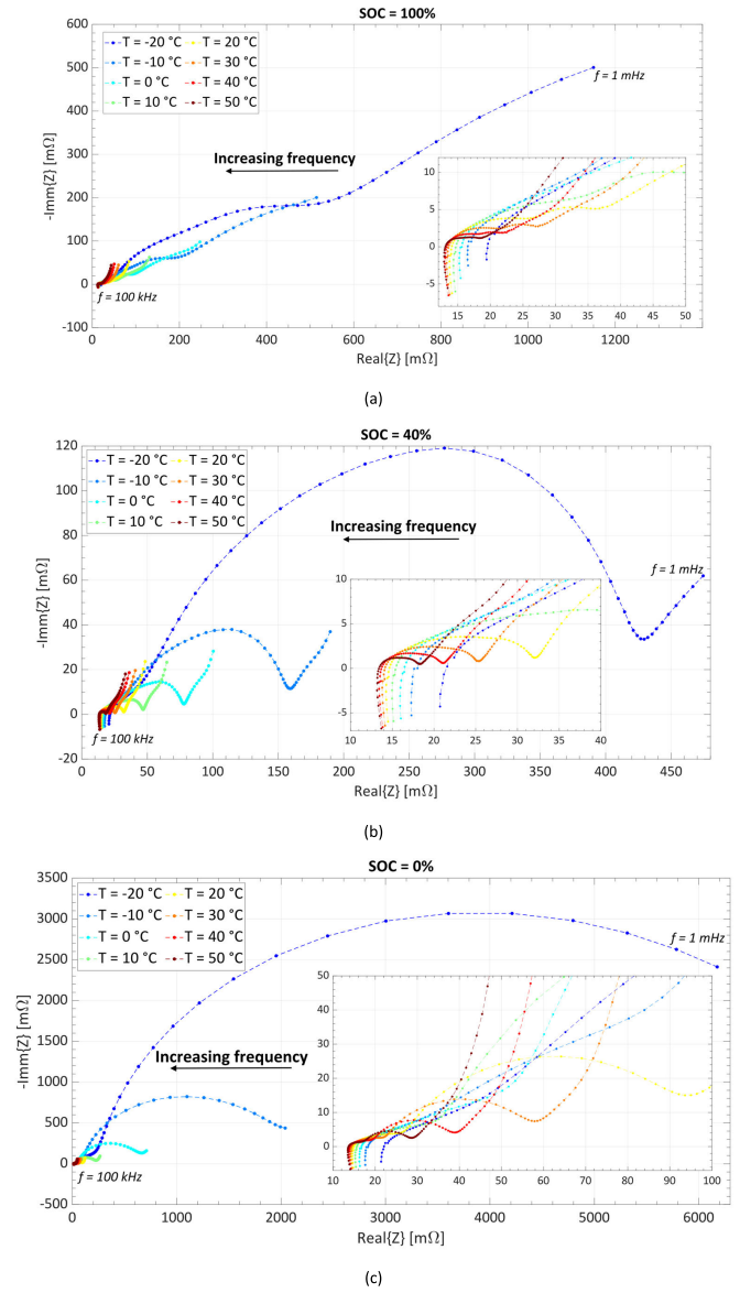
Fig. 4. Impedance spectroscopy at different temperatures. (a) Analysis with SOC = 100%. (b) Analysis with SOC = 40%. (c) Analysis with SOC = 0%.
