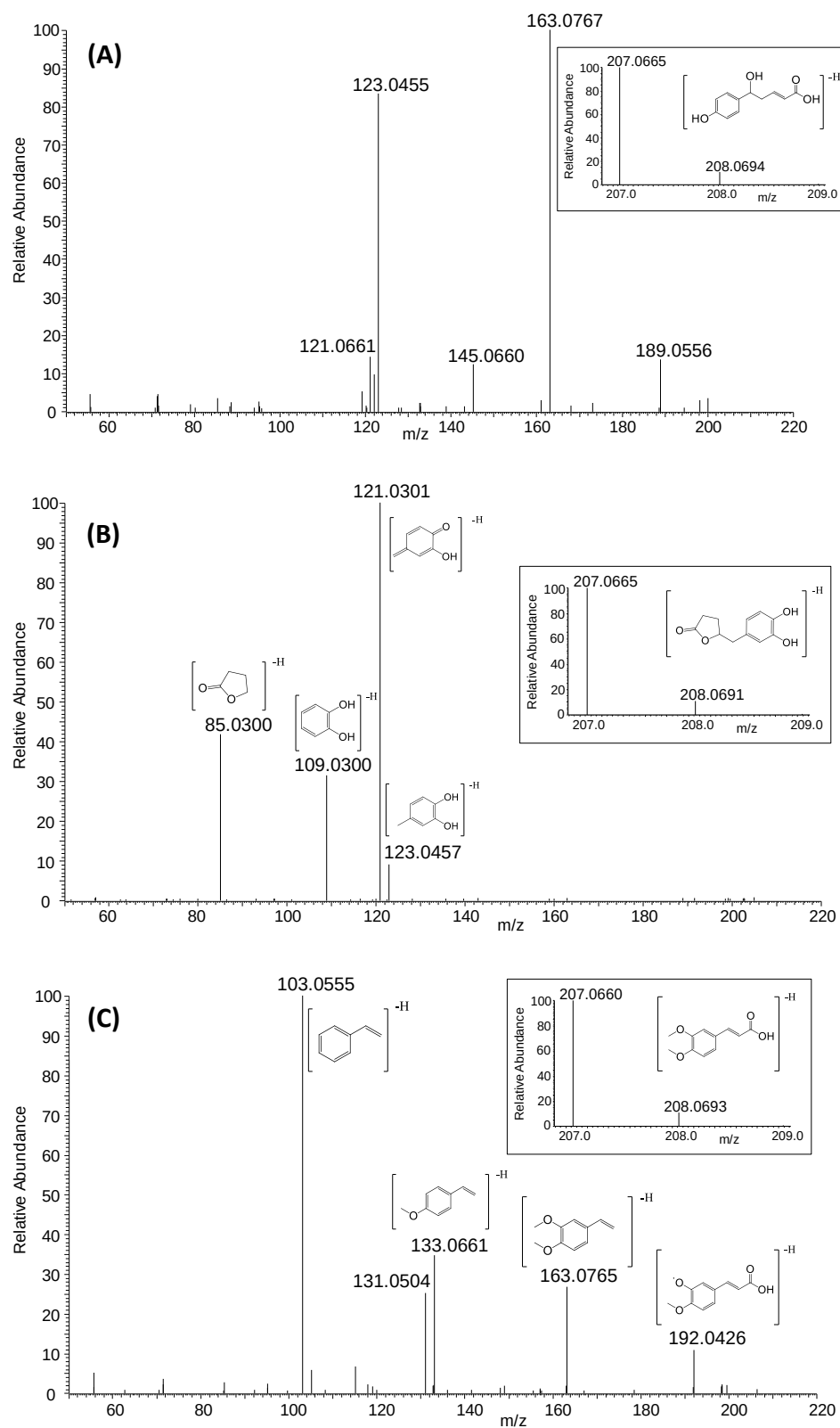
Figure 7. Isotopic profile and MS/MS spectrum of in-source fragment (m/z 207.0663) of peak 20 attributed to hydroxy-(hydroxyphenyl)-pentenoic acid sulphate (A), 3,4-dihydroxyphenyl-valerolactone reference standard (B) and 3,4-dimethoxycinnamic acid reference standard (C).
