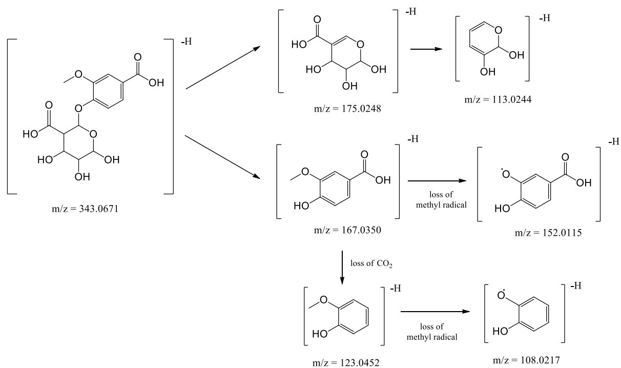
Scheme 1. Hypothesized structure and fragmentation scheme for peaks 1 and 7 ( [M-H]^- = 343.0663 ).
