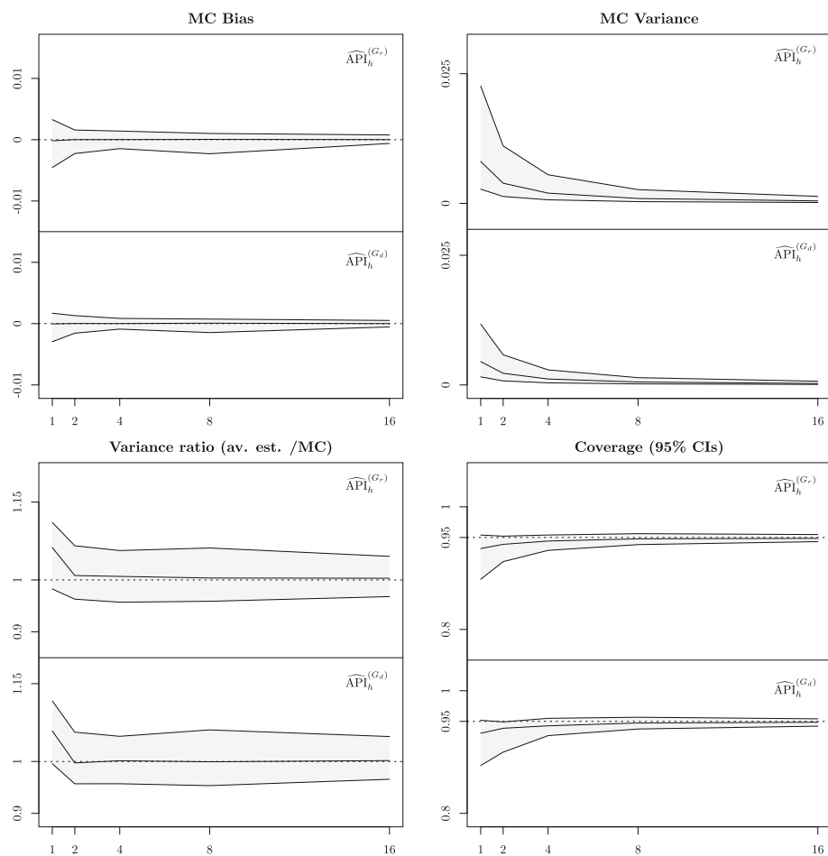
Fig. 1 Simulation results for \widehat{\text{API}}_h^{(G_d)} and \widehat{\text{API}}_h^{(G_r)}
