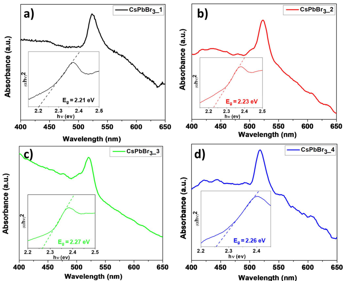
Fig. 8 UV-vis spectra of \text{CsPbBr}_3 microcrystals dispersed in ethanol synthesized from Cs(hfa) and the “Pb(hfa) 2 -glyme” precursor: (a) \text{CsPbBr}_3 _1, (b) \text{CsPbBr}_3 _2, (c) \text{CsPbBr}_3 _3, and (d) \text{CsPbBr}_3 _4. In the inset, Tauc plot (\alpha h\nu)^2 against photon energy ( h\nu ) of the \text{CsPbBr}_3 powders. The dotted lines represent the linear extrapolation of the E_g value.
