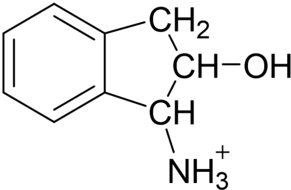
Scheme 2. 1-Amino-2-indanol fragment searched in the Cambridge Structural Database.
