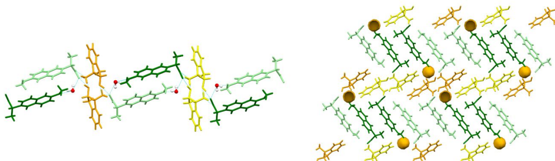
Figure 8. RS-AI_S-Nap_W crystal structure: ribbon motif (left) propagating along the b axis direction (dark and light green refer to the two independent naproxen anions, yellow and orange refer to the two independent indanol cations); isolated voids occupied by the water molecules (right).
