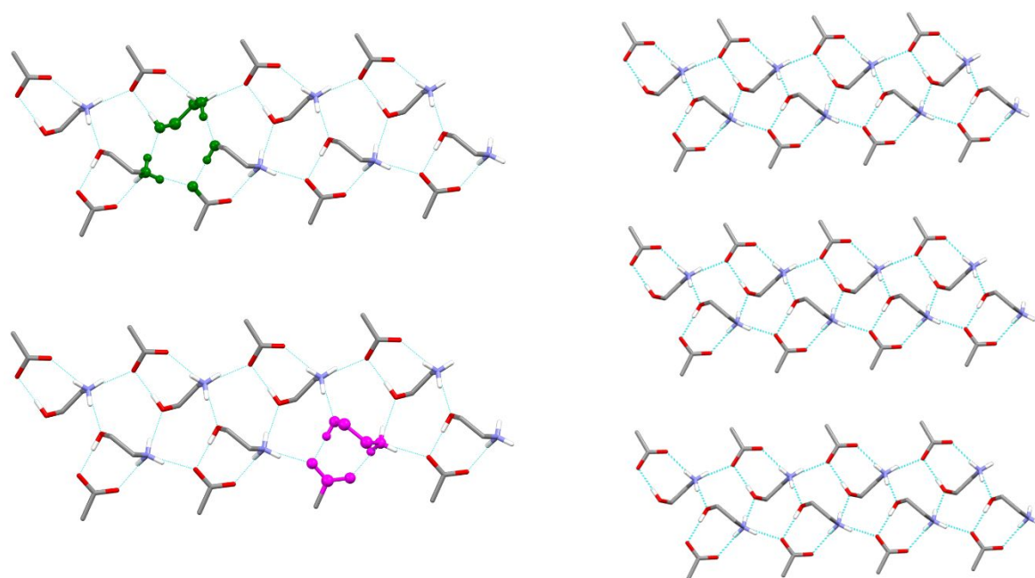
Figure 3. Schematic drawing of the H-bond network in the naproxen diastereomeric salts evidencing the R_2^2(9) (ball and stick, pink) and R_4^3(11) (ball and stick, green) H-bond motifs view along the a -axis direction. Left: columnar H-bond network; right: columns packing.
