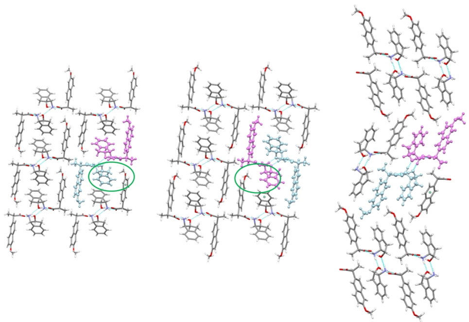
Figure 5. Crystal packing in SR-AI_S-Nap_A (left), RS-AI_S-Nap_A1 (middle) and RS-AI_S-Nap_A2 (right). The aromatic ring centroids help in evidencing the inter-column interactions; the green circle in SR-AI_S-Nap_A (left), RS-AI_S-Nap_A1 (middle) evidence the relative position of aminoindanol and methoxy group of adjacent columns (see text).
