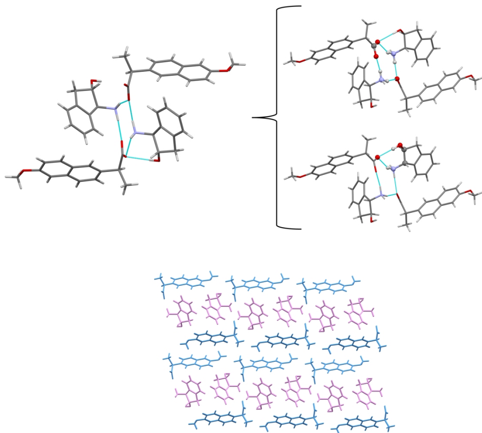
Figure 11. Crystal structure of (1S,2S)-trans-1-Aminoindan-2-ol (S)-2-(6-methoxy-2-naphthyl)propanoic acid (OKIQAA). Intermolecular H-bonds within each column viewed along the b-axis direction (top left); R3,4(10) and R1,2(7) motifs in the reinforced H-bonded tetramer (top right); crystal packing viewed along the b-axis direction made of alternating layers of naproxen and aminoindanol ions parallel to the ab crystal face (bottom).
