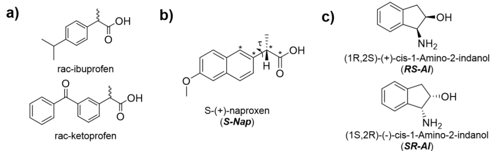
Scheme 1. a) Schematical drawing of Ibuprofen and Ketoprofen; b) Schematical drawing of (S)-(+)-Naproxen ( S-Nap ) with evidenced the atoms defining the torsion angle \tau ; c) Schematical drawing of (1R,2S)-(+)-cis-1-Amino-2-indanol ( RS-AI ) and (1S,2R)-(-)-cis-1-Amino-2-indanol ( SR-AI ).
