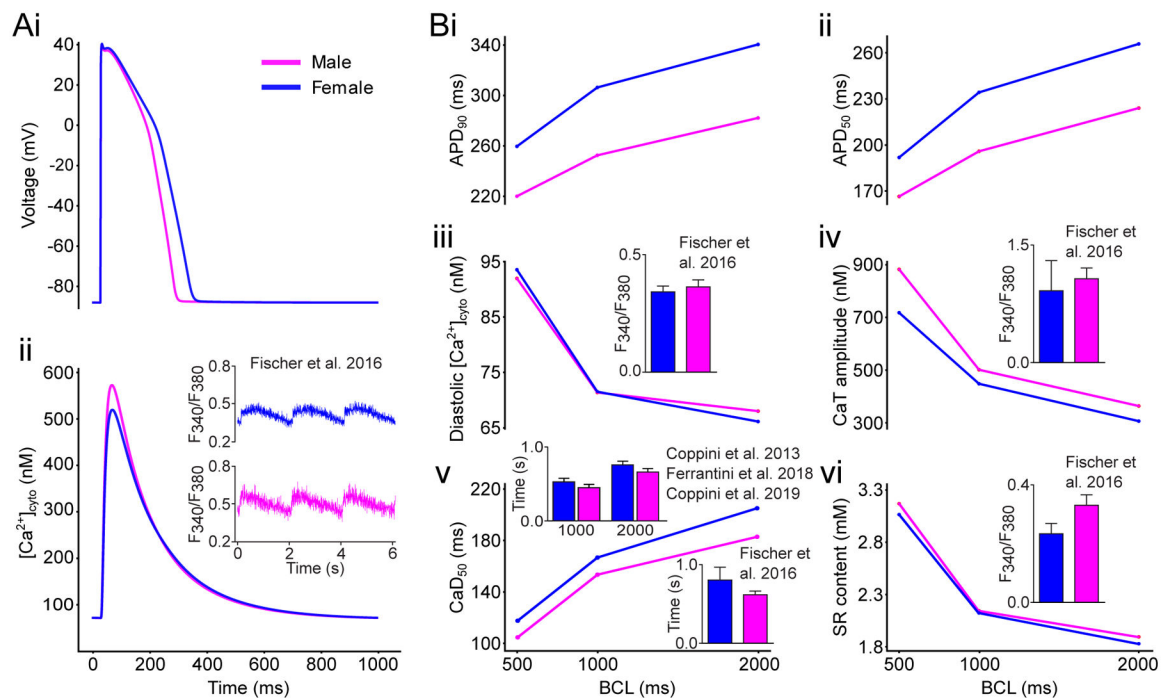
Figure 2: Sex-specific biophysical models of cardiac electrophysiology and \text{Ca}^{2+} handling.
