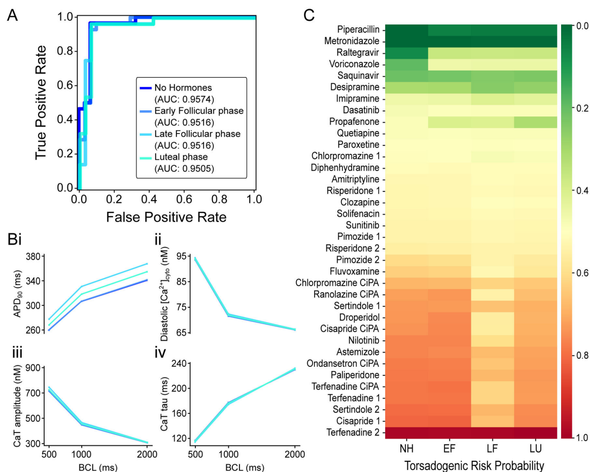
Figure 6: Effects of sex hormone fluctuations on female TdP classifier predictions.
