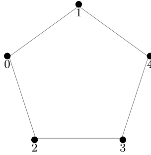
Fig. 1. The discrete model for the idealised version of the double bridge experiment
