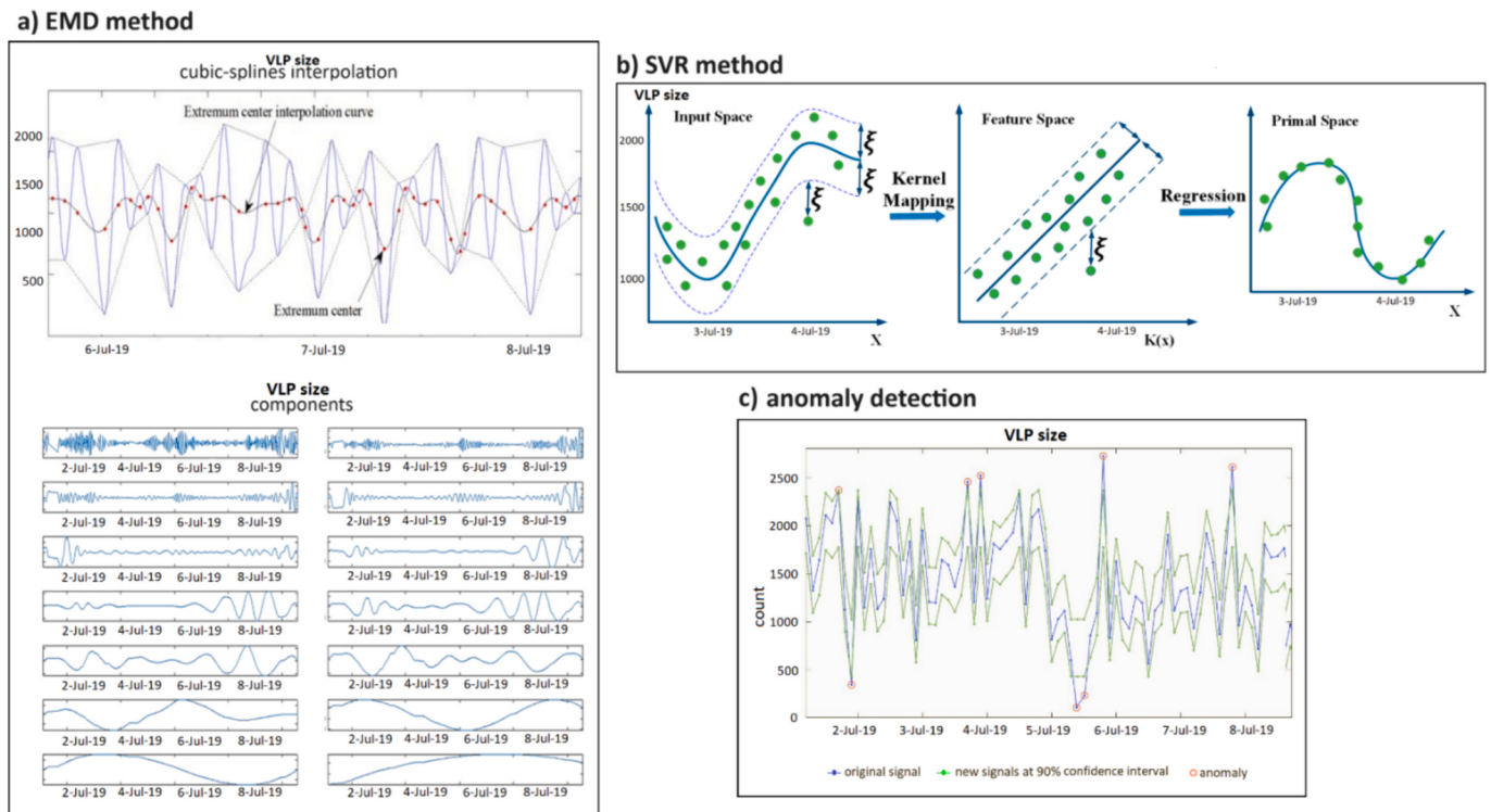
Fig. 4. Graphical visualization of the operations of the hybrid EMD + SVR method on a part of the VLP size signal (2 July 2019–8 July 2019). a) EMD application with a focus on the cubic-spline interpolation of the upper and lower local maxima and minima of the signal, the average signal obtained, and all the components in frequency. b) SVR application on the result from EMD method: creation of a regression model, by performing the least-squares fit technique, transposed into a high-dimensional dual space by using kernel mapping. c) Anomalies identification after hybrid method EMD + SVR: the anomalies (red circles) are the values of the original signal (blue line) beyond the two new boundary signals (green lines) from the EMD + SVR method at 90% of confidence interval.
