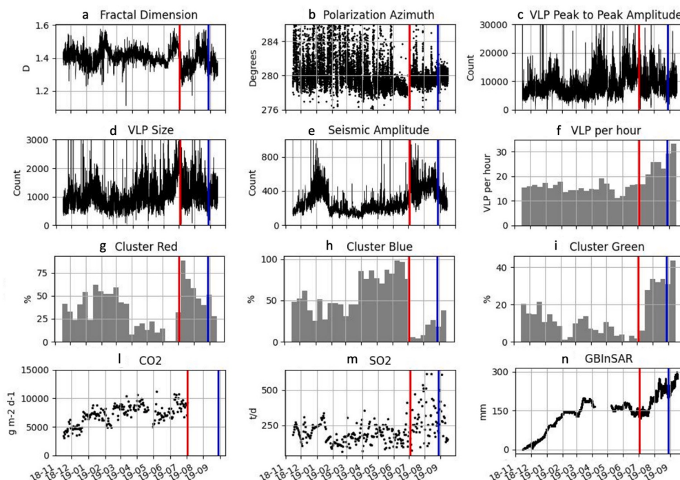
Fig. 3. The time series in the period 15 November 2018–15 September 2019. a) the fractal dimension of STRA east component; b) the azimuth of the polarization of the unfiltered STRA signal; c) the VLP peak-to-peak amplitude calculated on the STRA east component; d) VLP size calculated for the STRA east component; e) the Mean Square Seismic Amplitude of the 3-component signal module of the STRA station; f) VLP per hour is the daily VLP hourly rate; g) daily percentage of red cluster explosions; h) daily percentage of blue cluster explosions; i) daily percentage of green cluster explosions; l) daily soil CO 2 flux; m) daily SO 2 emission from the vents; n) GBInSAR displacement. The red and blue vertical lines indicate the 3 July and 28 August 2019 paroxysms, respectively.
