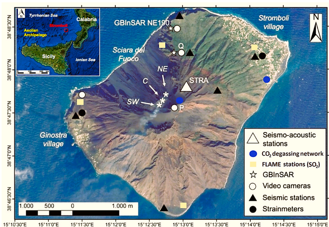
Fig. 1. Map of Stromboli Island (Italy) with the location of the INGV (Istituto Nazionale di Geofisica e Vulcanologia) and UniFi (University of Florence) monitoring stations: the black circles are the strainmeters; the black triangles are the seismic stations; the white circles indicate the position of the video cameras; the white stars are the GBInSAR devices; the yellow squares are the locations of the FLAME network stations; the blue circles are the stations of the soil CO 2 degassing geochemical network; the white triangle is the STRA seismic-acoustic station; the white asterisks are the main vent regions, with the white arrows indicating the SW, C and NE crater zones. P indicates the Pizzo Sopra la Fossa view site. The inset on the upper left displays the position of Stromboli island (red circle) in the southern Tyrrhenian Sea.
