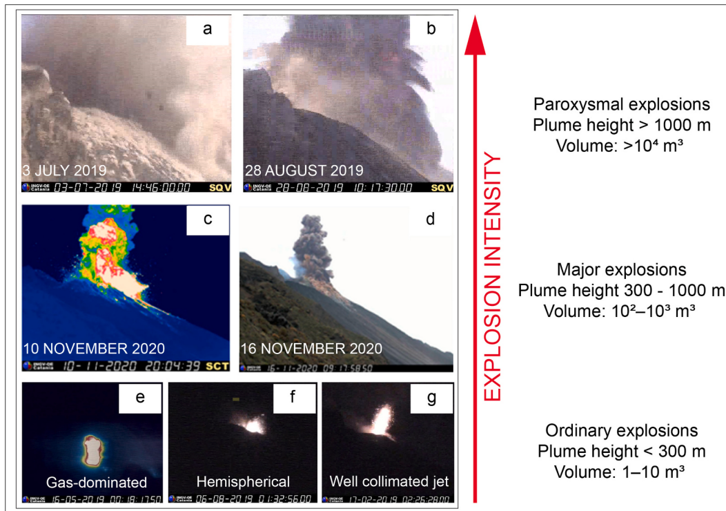
Fig. 2. Schematic representation of the explosive activity of Stromboli (modified after Calvari et al., 2021; Giudicepietro et al., 2022; Voloschina et al., 2023). a: eruptive column of the 3 July 2019 paroxysmal explosive event imaged by the SQV visible camera located on the east flank of the Sciara del Fuoco (SdF); vertical Field of View (FOV) is \sim 500 m. b: eruptive column of the 28 August 2019 paroxysmal explosive event imaged by the SQV visible camera located on the east flank of the SdF. c: thermal image from the SCT camera located at the northern edge of the SdF showing the eruptive column of the 10 November 2020 major explosion; vertical field of view \sim 300 m. d: eruptive column from the SCV visible camera located at the northern edge of the SdF of the 16 November 2020 major explosion; vertical FOV is \sim 600 m. e: thermal image from the SPT camera located at Il Pizzo (P, Fig. 1) showing from south-east a gas-dominated explosion; vertical FOV is \sim 300 m. f, g: side view of the hemispherical and well-collimated jet from the ordinary explosions imaged from the SQV visible camera.
