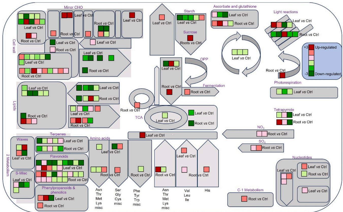
Fig. 4. MapMan pathway distribution based on differentially expressed transcripts (DETs) for the pairwise comparisons “Root under chromium stress versus Root under unstressful control conditions” [= Root vs Ctrl] and “Leaf under chromium stress versus Leaf under unstressful control conditions” [= Leaf vs Ctrl]. DETs involved in primary and secondary metabolism in response to chromium stress in leaves and root tissues. The log(fold change) of each DET (square) is expressed in a colorimetric scale (from red box = up-regulated to green box = down-regulated).
