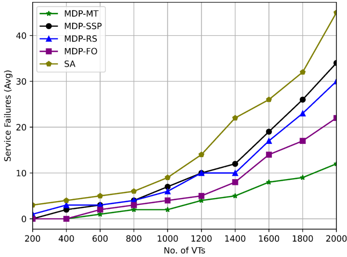
Fig. 9. Avg. No. of service failures.
