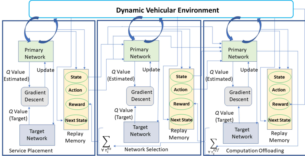
Fig. 3. Proposed deep Q-learning solution.
