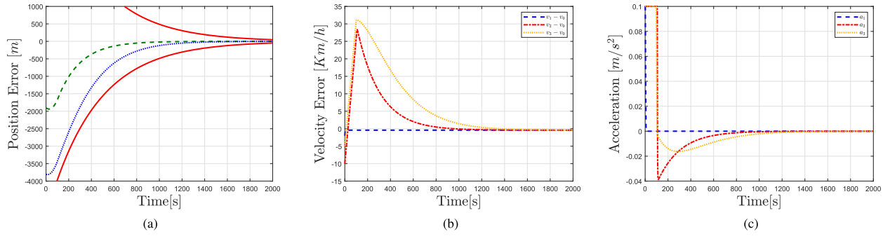
Fig. 6. Couplings creation and maintenance. (a) Time history of the position errors (green dashed line: r_2(t) - r_1(t) - h_{21}v_0 - d^{st} ; blue dotted line: r_3(t) - r_1(t) - h_{31}v_0 - d^{st} ), exponential envelopes are shown in red). (b) Time history of the speed error with respect to the reference. (c) Time history of the train accelerations.
