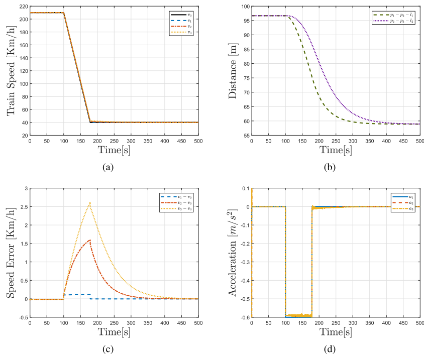
Fig. 7. Emergency Braking. (a) Time history of speed profile. (b) Time history of the bumper-to-bumper distance between the trains. (c) Time history of the speed error. (d) Time history of the train accelerations.
