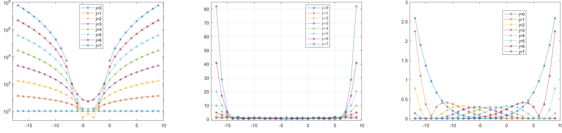
Figure 2: Behaviour of the coefficients generating the monomials x^j (left), the Chebyshev polynomials T_j (center), the Bernstein polynomials B_j^7 (right), for j = 0, \dots, 7 . The kernel \varphi is the B-spline of order 8.
