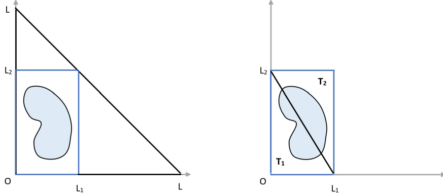
Figure 1: The domain D of the algebraic curve is contained inside the rectangular region \Omega = [0, L_1] \times [0, L_2] , which we embed inside a triangle with vertices (0,0) , (L,0) , (0,L) with L = L_1 + L_2 (left) or which we split into two triangles (right).
