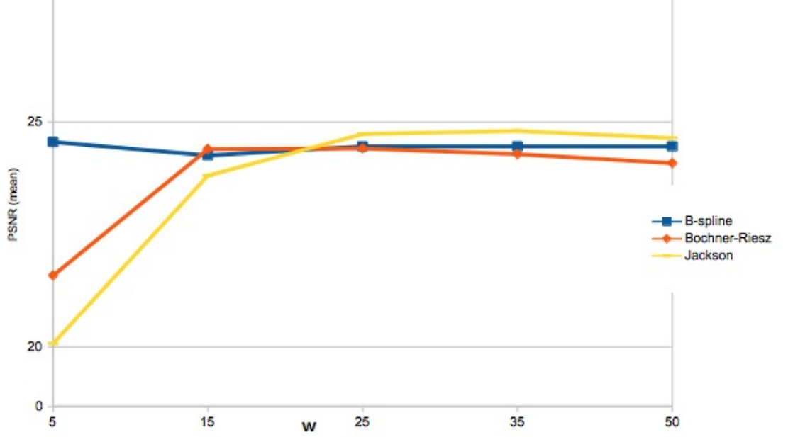
Figure 6: Trend of PSNR after the reconstruction of the images by the S-K algorithm. The saturation process occurs as w increases.
