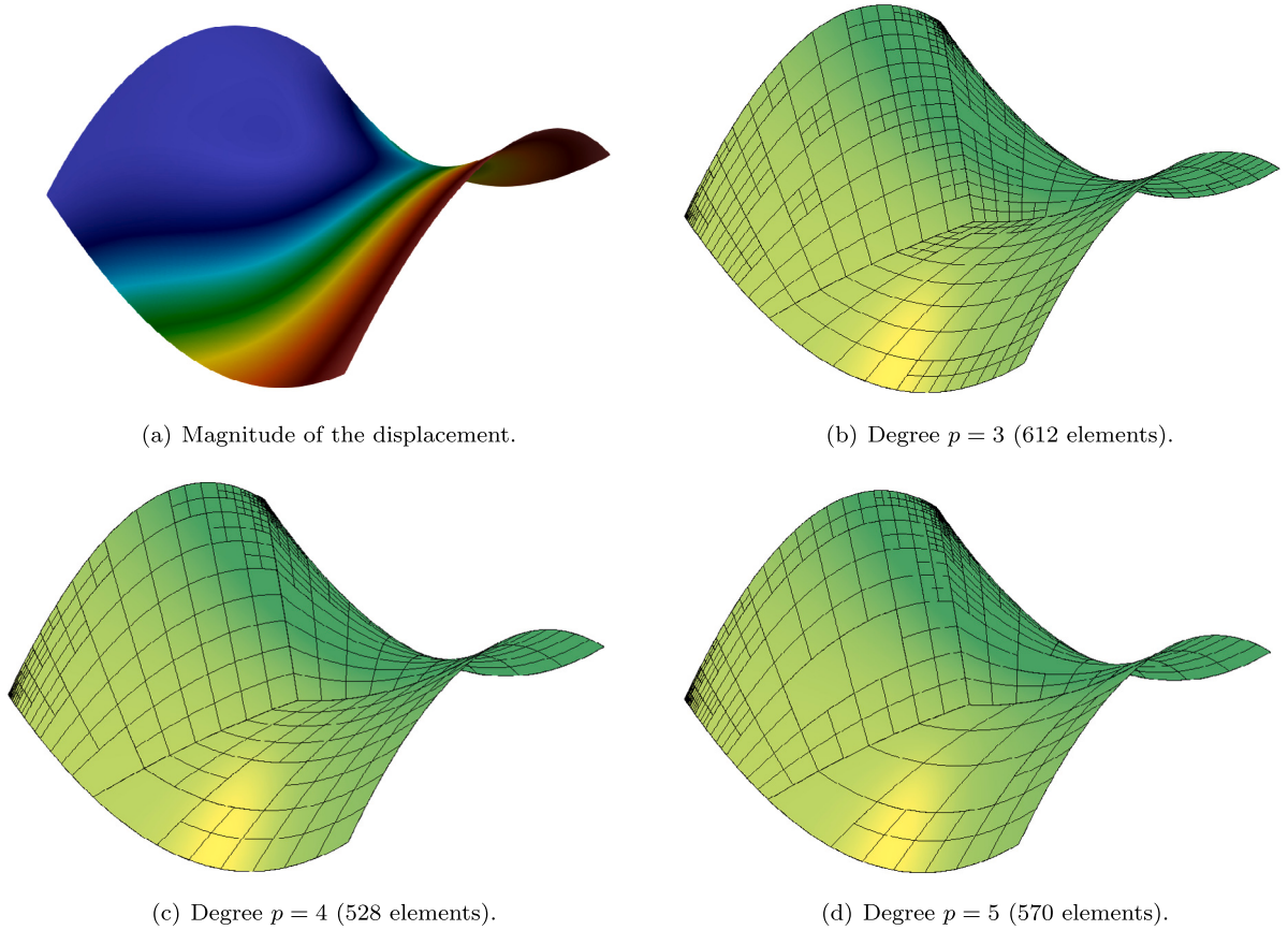
Fig. 10. Hyperboloid Kirchhoff-Love shell. Reference solution, and adaptive meshes at the last step.
