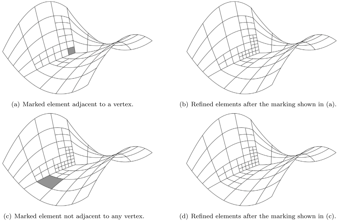
Fig. 1. If an element adjacent to a vertex is marked for refinement, highlighted in dark gray in (a), all the elements in its vertex-patch neighborhood must be also refined (b). If the marked element is not adjacent to any vertex (c), no additional elements need to be refined (d), even if the marked element belongs to the support of vertex basis functions.
