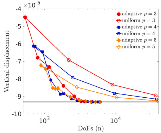
(b) Vertical displacement of point \mathbf{A} = (0.5, 0, -0.25) .
