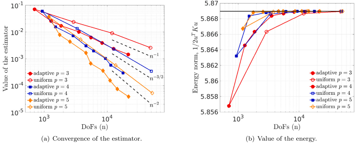
Fig. 8. Paraboloid Kirchhoff-Love shell. Convergence of the estimator and value of the energy.
