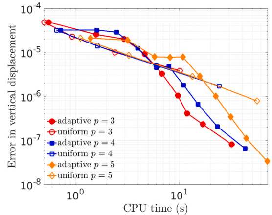
(b) Vertical displacement of point \mathbf{A} = (0.5, 0, -0.25) .
