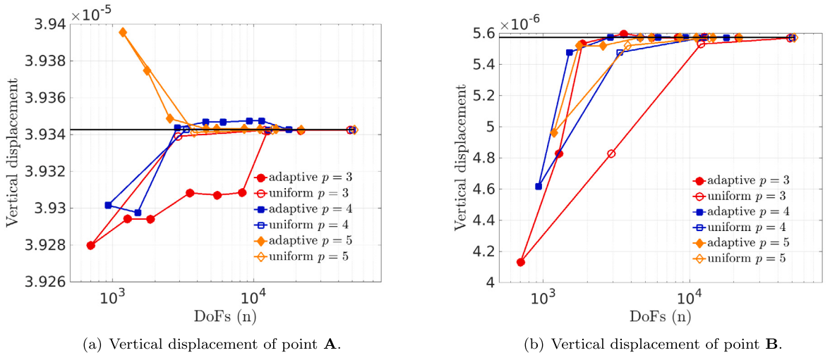
Fig. 9. Paraboloid Kirchhoff-Love shell. Vertical displacement for points A and B.
