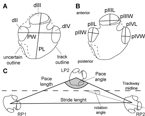
Fig. 2. Measurements. The track used as reference is the neotype of Rhinocерipeda tasnadyi (Kordos, 1985) redrawn by the authors. A. Perissodactyl pes track (right). Track length (PL) and width (PW), labelling of digits and explanation of the lines used. B. Perissodactyl digit measures. Digit II length and width (pII, pIIW), digit III length and width (pIII, pIIIW), digit IV length and width (pIV, pIIIVW). C. Trackway parameters.
