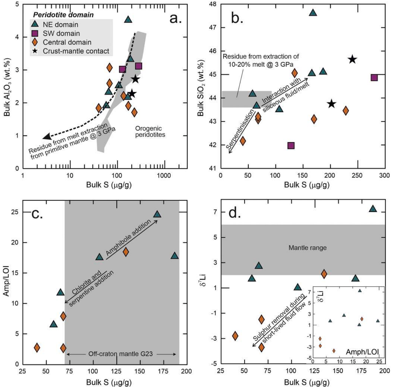
Fig. 6. Relationships of bulk-rock sulfur abundances ( \mu g\ g^{-1} ) in Ulten Zone peridotites (from Consuma et al., 2021) with various compositional and mineralogical parameters (from Gudelius et al., 2019; this study). a. Bulk-rock sulfur (note log scale) vs. Al_2O_3 concentration. Shown for comparison are the quantitatively modelled trend for melt extraction from a primitive mantle source at 3 GPa and the field for orogenic peridotites world-wide from Aulbach et al. (2016). Bulk-rock sulfur vs. b. SiO_2 concentration, possibly indicating addition during interaction with high- P siliceous fluid, and c. the ratio of amphibole modal abundance over Loss-On-Ignition (LOI) values, as a measure of the abundance of amphibole (Amph) vs. chlorite + serpentine. In b., grey field encompasses range of concentrations in a residue of 10–20% melting commencing at 3 GPa (S from Aulbach et al., 2016; SiO_2 from Herzberg, 2004), consistent with melt fraction and melting pressure estimates for Ulten Zone peridotites of Ionov et al. (2017) and Gudelius et al. (2019). In c., range of sulfur concentrations in off-cratonic lithospheric mantle from Gibson and McKenzie (2023; G23). d. Bulk-rock sulfur concentration vs. \delta^7Li (in ‰), interpreted to reflect the transient ingress of crustal fluid, with addition of fluid-mobile elements including Li, and removal of the fluid source before isotopic equilibration could take place, leading to enrichment in ^6Li over ^7Li . Inset shows \delta^7Li vs. Amph/LOI, confirming the exhumation-related nature of this event, with formation of chlorite and serpentine at the expense of amphibole. Mantle \delta^7Li range from Ionov and Seitz (2008).
