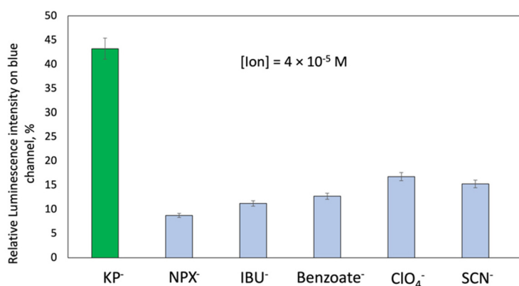
Fig. 7 Relative luminescence intensity of membrane Mb5 sensing spots on the blue channel in the presence of equal amounts of KP - , naproxen (NPX - ), ibuprofen (IBU - ), benzoate (Benzoate - ), ClO_4^- and SCN^- interfering anions. [Ion] = 4 \times 10^{-5} M, pH = 7.0, Tris 0.005 M, and \lambda_{exc} = 365 nm.
