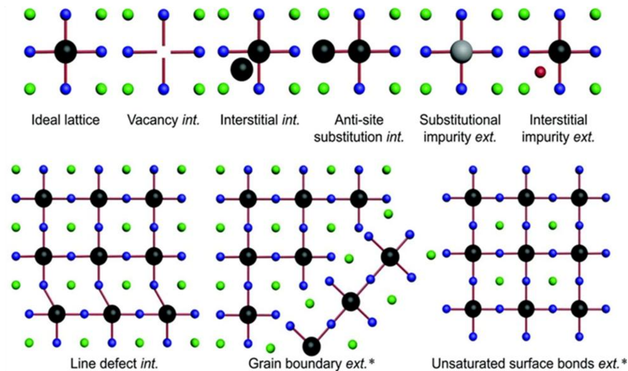
Figure 2.5. Schematic representation of an ideal PVK lattice with AMX_3 formula and the possible defects in it (Green, black and blue dots represent the A-, M- and X-site ions respectively; Red and grey dots represent the impurities) 78 .
