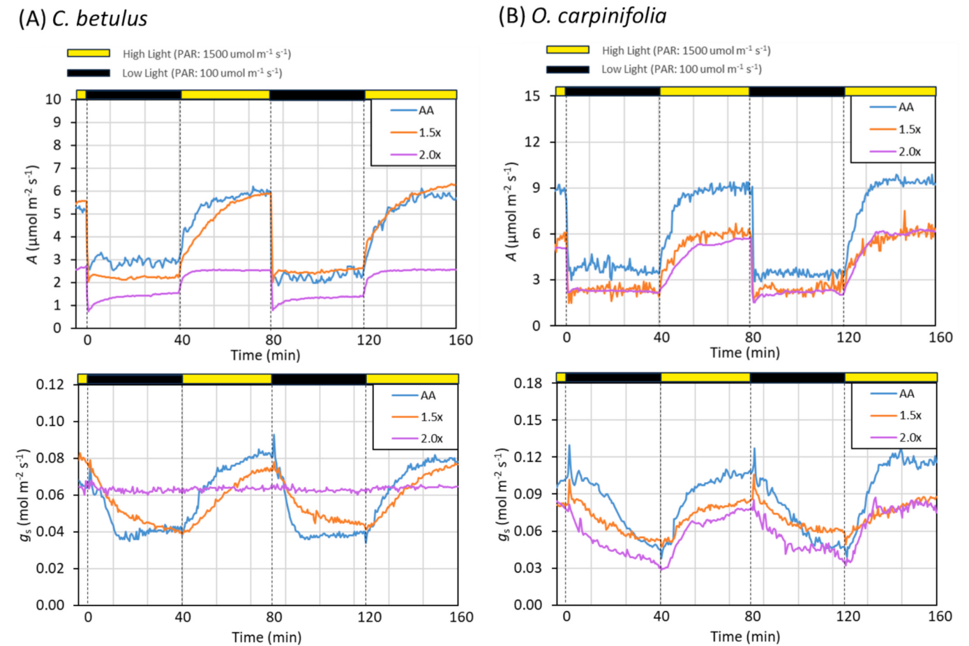
Fig. 1. Example of dynamic response of net photosynthetic rate (A) and stomatal conductance ( g_s ) to changes in light intensity (yellow horizontal bars: PAR = 1500 \mu\text{mol m}^{-2} \text{s}^{-1} ; black horizontal bars: PAR = 100 \mu\text{mol m}^{-2} \text{s}^{-1} ) for C. betulus (CB) and O. carpinifolia (OC) plants exposed to three levels of O_3 (ambient air, AA; 1.5 times ambient ozone concentration, 1.5 \times AA; twice ambient ozone concentration, 2.0 \times AA).
