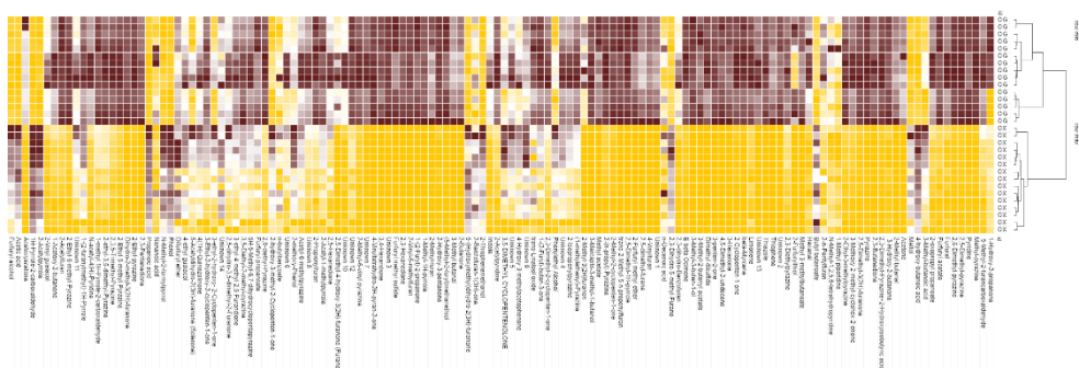
Figure 1. Coffee volatilome heatmap of good and oxidized samples
