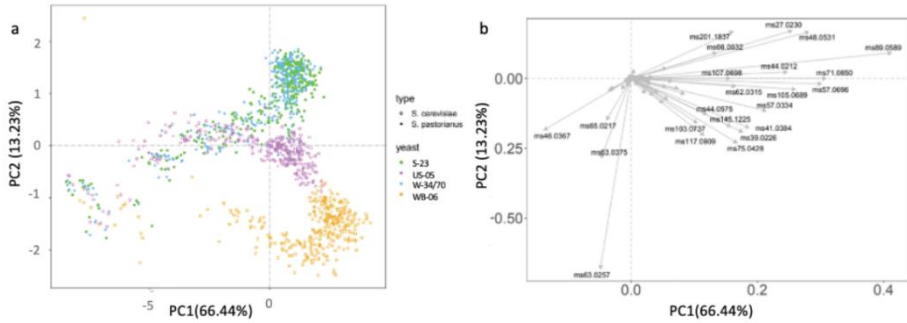
Figure 2. Score plot of the principal component analysis (PCA) of volatile organic compound (VOC) (a) and loading plot of PCA of the mass peaks (ms) (b) for yeast: S. cerevisiae (US-05 and WB-06) and S. pastorianus (W-34/70 and S-23). Samples were measured every 6 hours over a 5-day incubation at 20°C using PTR-ToF-MS
