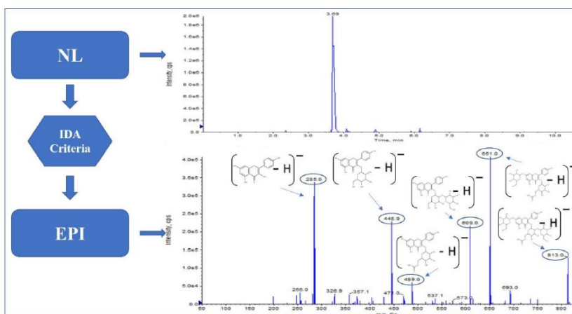
Figure 1. Kaempferol-glucosyl-(1->2)-(6''-acetylgalactoside)-hexoside fragmentation pattern in Saffron
