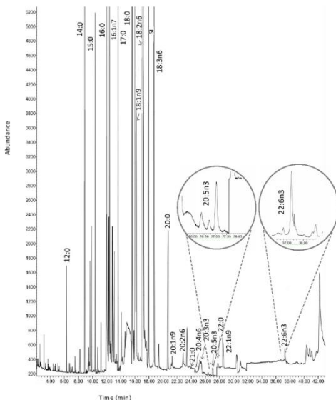
Figure 1. Example of chromatogram of the FAs composition of Acheta domesticus fed with feed containing 20% of P. palmata
