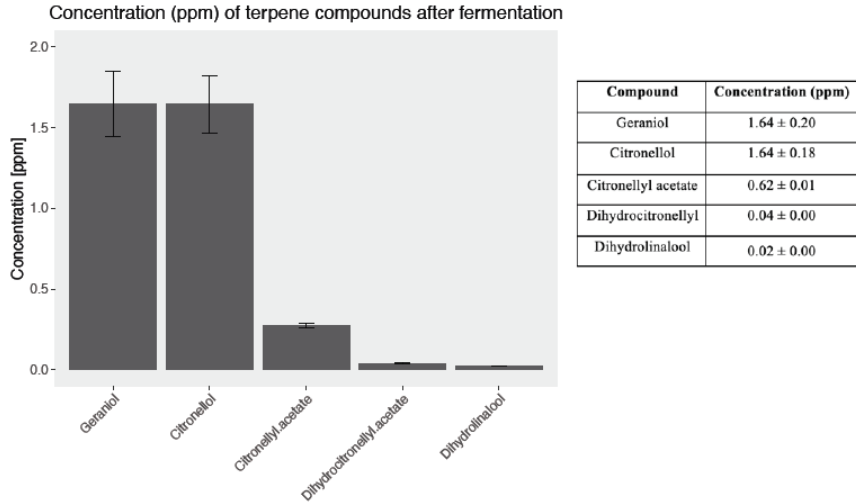
Figure 1. Biotransformation of (10 ppm) geraniol by SafAle US-05 ( S. cerevisiae ) yeast. Samples were measured after 5-days incubation at 20°C using SPME GC-MS. The mean concentration of the spiked compound and the terpenes produced are displayed. The error bars represent the standard deviation of three replicates
