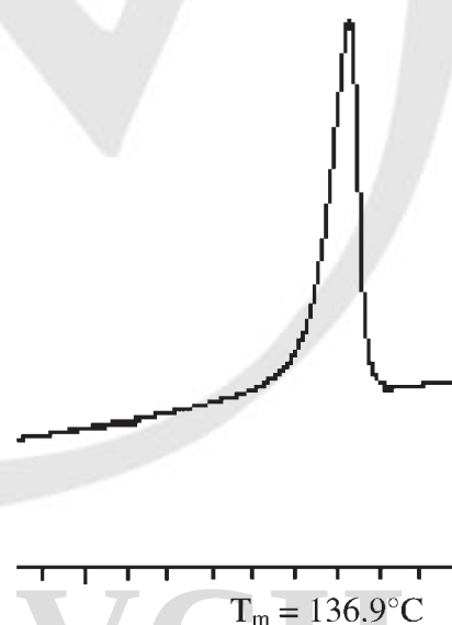
Figure 4. DSC spectrum of polyethylene obtained at 60 °C in the presence of 1 /MAO (Table 1, run 2).
