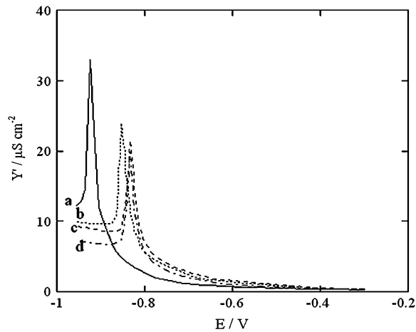
FIGURE 1 Y' versus E plots at a tBLM in aqueous solution of 0.1 M KCl and 0.7 \mu\text{M} SLN, recorded after 15 (a), 45 (b), 90 (c), and 120 min (d) from SLN addition to the 0.1 M KCl solution.
