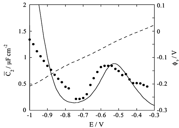
FIGURE 10 Plot of the capacity \bar{C}_2 of the lipid bilayer against E for a tBLM incorporating SLN from its 0.7 \mu\text{M} solution in aqueous 0.1 \text{ M KCl} . Solid circles are experimental values, and the solid curve was calculated from the model for the same values as in Fig. 8. The dashed curve is the curve of the transmembrane potential \phi_2 against potential calculated from the model.
