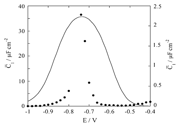
FIGURE 9 Plot of the capacity \bar{C}_1 of the hydrophilic spacer against E for a tBLM incorporating SLN from its 0.7 \mu\text{M} solution in aqueous 0.1 M KCl. Solid circles are experimental values, and the solid curve was calculated from the model for C_0 = 4 \mu\text{F cm}^{-2} , C_1 = 7 \mu\text{F cm}^{-2} , C_2 = 1 \mu\text{F cm}^{-2} , \chi_1 = -0.250 \text{ V} , a = 50 \text{ V}^{-1} , \Delta = -0.050 \text{ V} , K_{+,1} = K_{-,1} = 5 \times 10^{-3} , K_{+,2} = 1 \text{ cm}^3 \text{ mol}^{-1} , and for K_{-,2} = 1 \times 10^4 \text{ cm}^3 \text{ mol}^{-1} . The left-hand vertical axis refers to the solid circles, the right-hand one to the solid curve.
