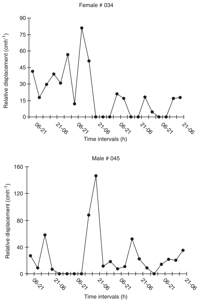
Figure 1. Relative displacement (in \text{cm h}^{-1} ) with time in two radio-tracked crayfish (numbered from the frequency of their radio-transmitters, in kHz).
