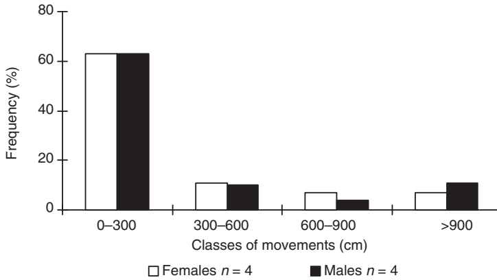
Figure 2. Frequency distributions (in %) of classes of movements (in cm) in the two sexes between two subsequent radio-fixes.
