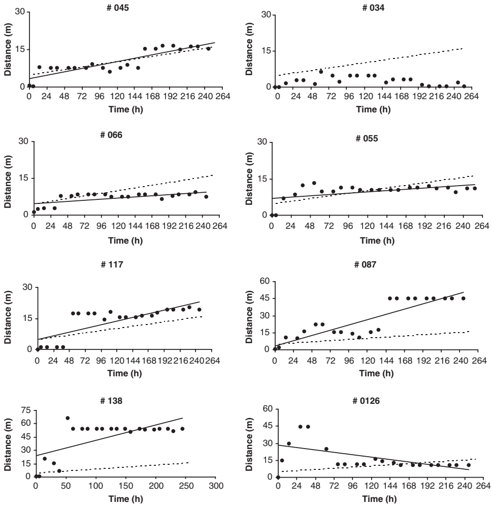
Figure 3. Observed (continuous lines) and expected (dashed lines) dispersal (distance in m from the starting point vs. time in h) for every crayfish (numbered from the frequency of its radio-transmitter, in kHz). See Table III for details.
