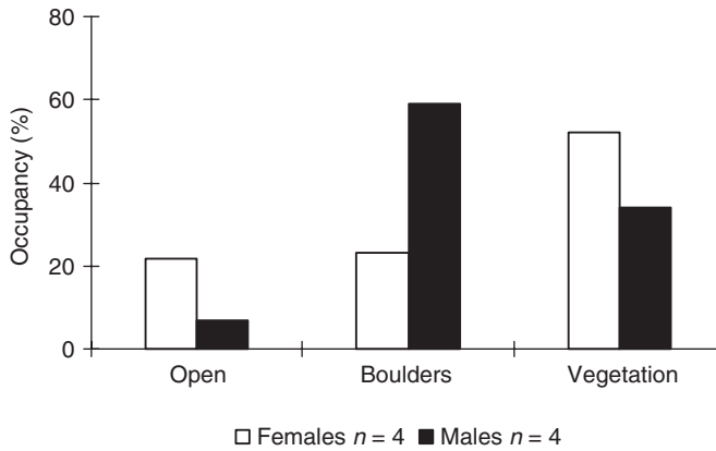
Figure 4. Frequency distributions (in %) of occupancy of three microhabitats (open, boulders, and vegetation) by the two sexes.
