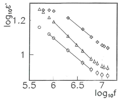
FIG. 5. The \log_{10}(\epsilon') versus \log_{10}(f) curves are shown for samples with \phi = 0.130 (open circles), 0.145 (open triangles), and 0.200 (open crosses). The straight lines represent the fitting results [see Eq. (8)].
