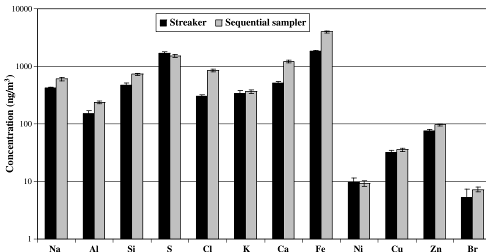
Fig. 2. Average 24-h concentration of some elements obtained by daily samples and streaker films in the PM 10 fraction.
