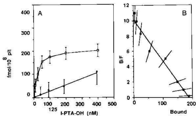
Fig. 3. (A) Saturation curve for [ 125 I]PTA-OH binding to washed human platelets at 20 °C (○) total binding; □ specific binding; ● non-specific binding (n = 12). (B) Scatchard analysis of the specific binding ( B_{max} = 198 \pm 63 fmol/10 8 platelets, K_d = 21.5 \pm 7.2 nM).
