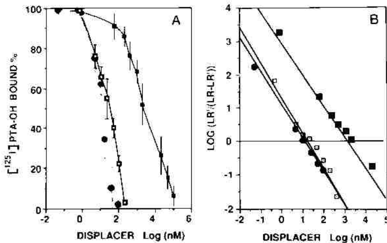
Fig. 5. (A) Displacement of specific [ ^{125}\text{I} ]PTA-OH binding by increasing concentrations of ONO11120 (□), U46619 (●) and picotamide (■). Data points represent the means of triplicate determinations in at least 10 independent experiments. (B) Hill plot of the displacement curves. K_{\text{i}} values, calculated according to Cheng and Prusoff (1973), were 19 \pm 4 nM for ONO11120 ( n = 10 , n_{\text{Hill}} = 0.942 \pm 0.096 ), 17 \pm 3 nM for U46619 ( n_{\text{Hill}} = 0.943 \pm 0.096 , n = 10 ) and 1472 \pm 321 nM for picotamide ( n_{\text{Hill}} = 0.970 \pm 0.075 , n = 9 ).
