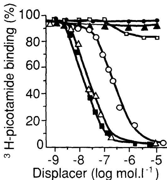
FIG. 4. Displacement of the specific [ ^3\text{H} ]methylene-picotamide binding by increasing concentrations of different compounds. Solid squares = U46619 (9,11-dideoxy-11 \alpha , 9 \alpha -epoxymethano-prostaglandin F _2 ); empty triangles = ONO11120 (9,11-dimethylmethano-11,12-methane-16-phenyl-13,14-dihydro-13-aza-15-tetranor-TXA _2 ); empty circles = picotamide; empty squares = TXB _2 ; solid triangles = PGE _2 ; solid circles = PGI _2 (from ref. 41 with permission).
