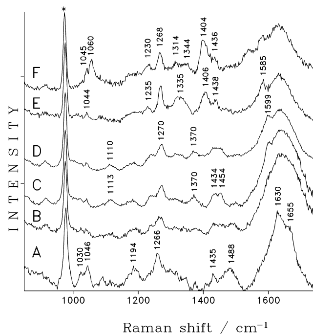
Fig. 4. Raman spectra of \text{Cu}^{\text{II}} -AcHGHG in aqueous solutions at different pH: 2.0 (A); 4.75 (B); 5.55 (C); 6.45 (D); 8.4 (E); 12.0 (F). Dotted band at \sim 980\text{ cm}^{-1} refers to \text{SO}_4^{2-} ion vibration.
