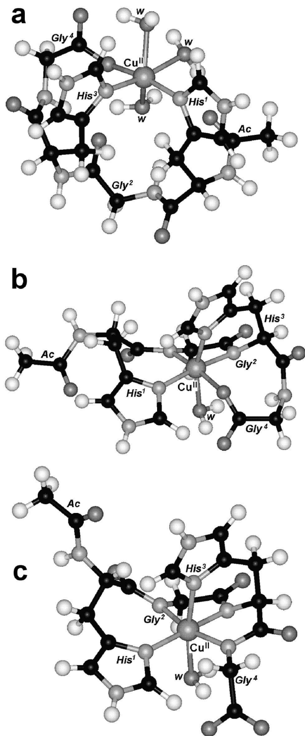
Fig. 5. Optimized structures of the main HL/Cu II complexes at (a) pH 5.6, (b) pH 7.0 and (c) pH > 8, obtained from PM3(tm) semi-empirical calculations.
