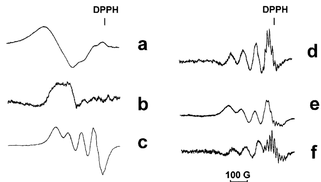
Fig. 2. X-band EPR spectra of the Cu II –AcHG HG system (ligand-to-metal ratio =1:1) at RT. pH=2.9: (a) first derivative, (b) second derivative. pH=8.4: (c) first derivative, (d) second derivative. pH=10: (e) first derivative, (f) second derivative.
