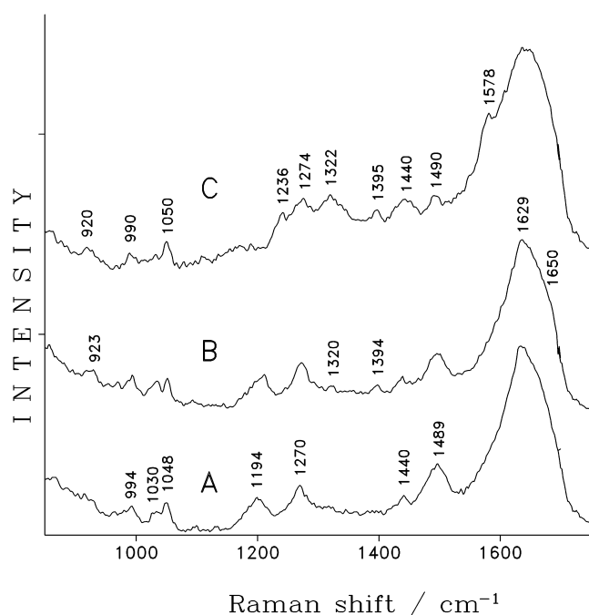
Fig. 3. Raman spectra of AcHGHG in aqueous solutions at different pH: 2.9 (A); 5.1 (B); 8.7 (C).
