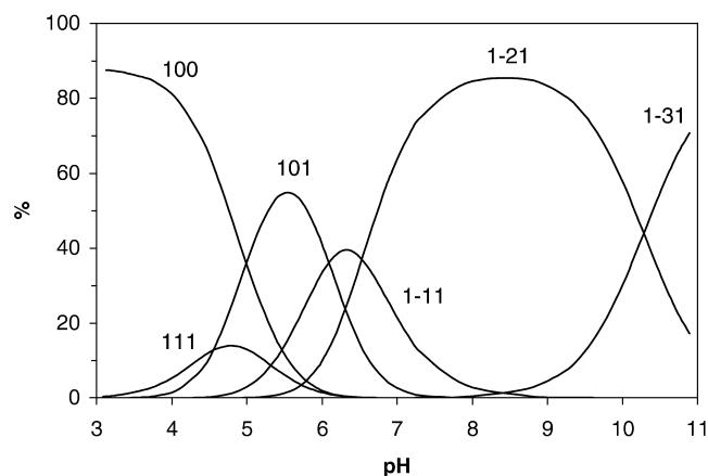
Fig. 1. Computed species distribution curves for the Cu II –HG HG system (ligand-to-metal ratio 1:1) at 25 °C in 0.1 M NaCl. Each species M p H q L r is indicated by subscripts p, q and r.
