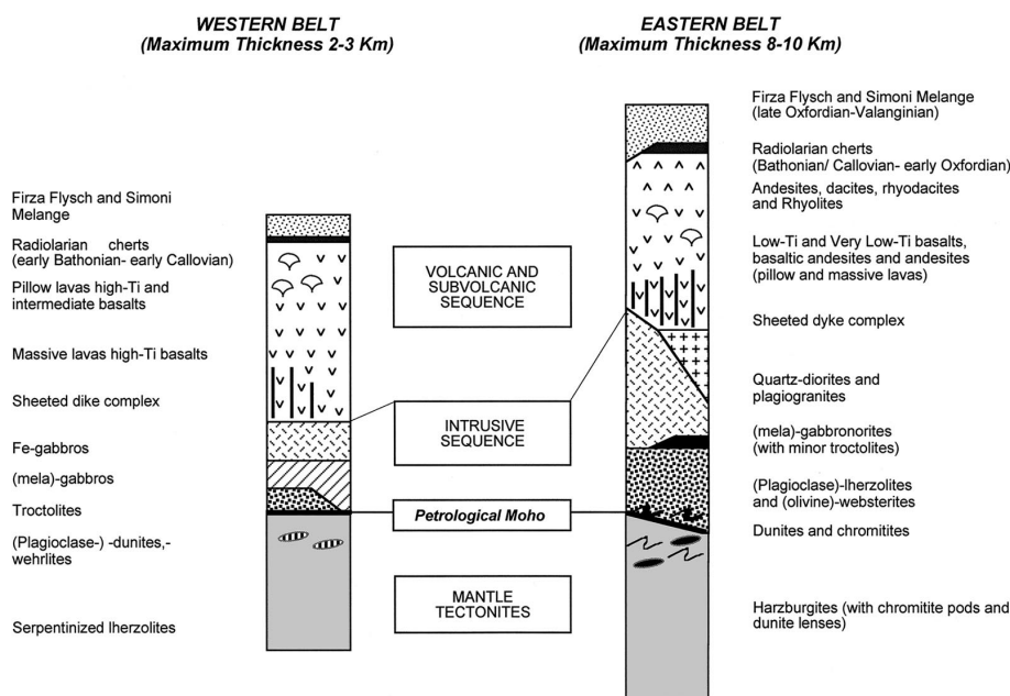
Fig. 4 - Generalised stratigraphy of the ophiolite sequences for the Western and Eastern belt (Modified after Bortolotti et al., 1996).
