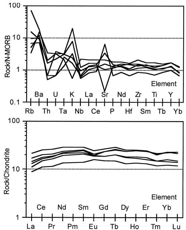
Fig. 3 - Incompatible element and REE patterns for representative Triassic MORBs from the sub-ophiolite mélange. Modified from Bortolotti et al. (2004). Normalization values are from Sun and McDonough (1989).
