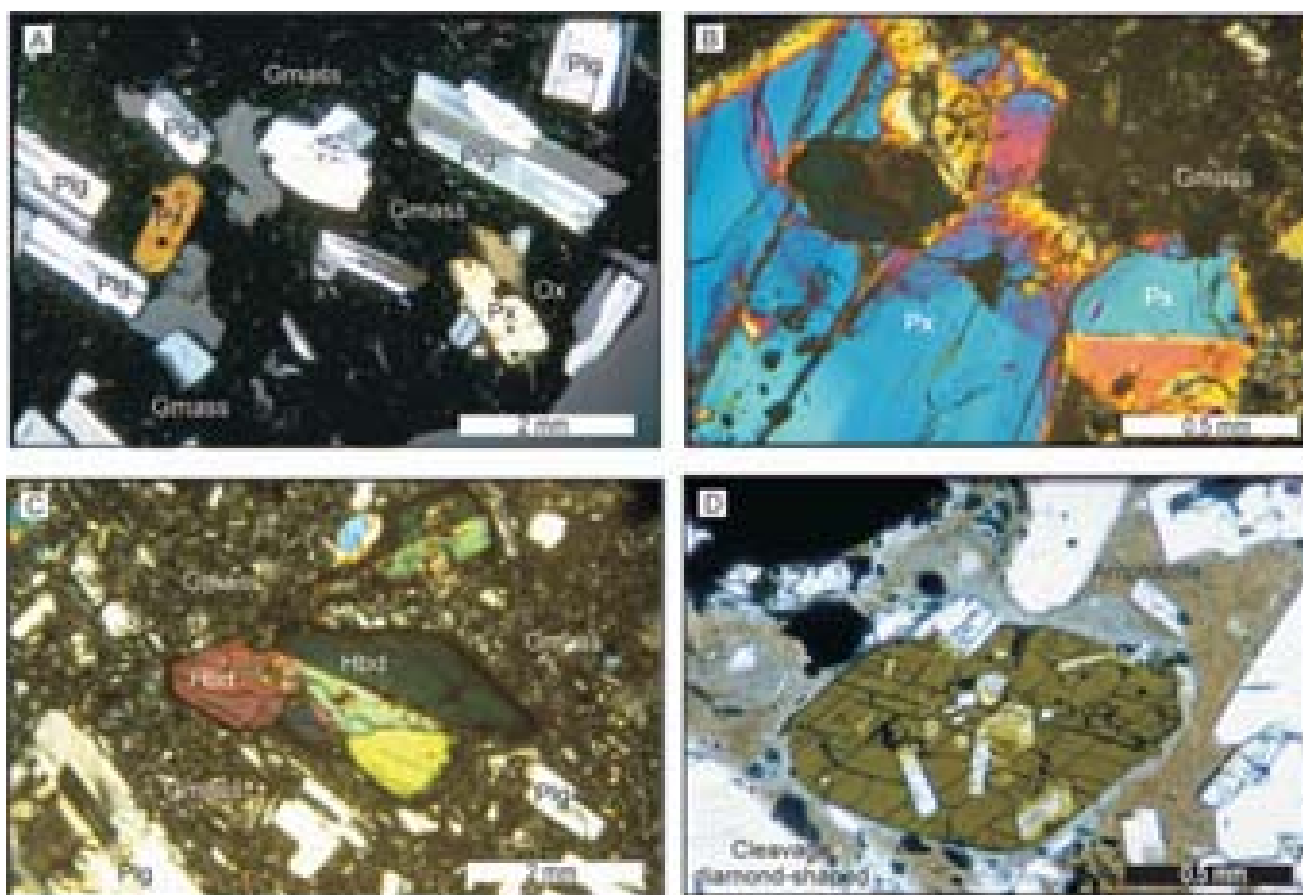
Fig. 4. Photomicrographs showing main mineral phases from lava flow samples of Chichuj volcano. A) Aligned plagioclase with subhedral-anhedral forms in a fine-grained groundmass. B) Pyroxene crystals with subhedral and euhedral forms, slight fractured, and showing sector and patchy zoning. C-D) Hornblende with characteristic cleavage, diamond-shaped sections, subhedral and euhedral forms, crystals with slight reaction rims of black color by the presence of Fe-Ti oxides.
