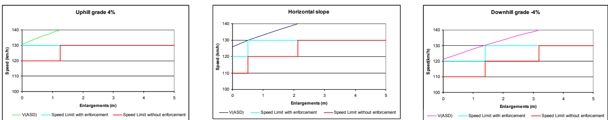
Figure 23: Required speed limit as a function of the enlargement actually realized for type A road most critical right-hand bend (R=964m)
