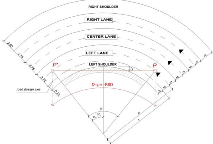
Figure 2: Cross section enlargement ( \Delta ) required in Two Carriageways Roads left-hand bends
