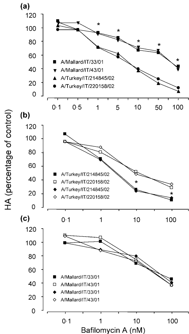
Fig. 1. Effect of treatment with bafilomycin A on virus replication on MDCK cells. (a) Virus growth curves of duck and turkey H7N3 viruses in the presence of bafilomycin A throughout the 4 day replication period. (b and c) Virus growth curves of turkey and duck viruses in which bafilomycin A treatment was restricted to 2 h of virus adsorption. Treatments were conducted at 4 °C to estimate the effect on virus attachment (open symbols) and at 37 °C to measure effect on viral internalization (filled symbols), respectively. Virus growth is expressed as the relative levels of HA found in the supernatant fluids of virus grown in the presence of bafilomycin A compared with that obtained in its absence. Values shown are the mean of three independent experiments. Asterisks indicate that inhibition of duck viruses was significantly different from that of the viruses isolated from turkeys and that inhibition of turkey viruses, under treatment restricted to the virus adsorption, was significantly affected by the temperature at which was conducted (Student's t -test) at P < 0.05 .
