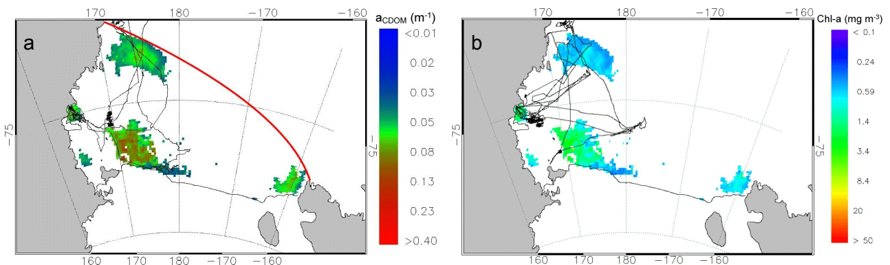
Figure 3: a_{\text{CDOM}} (a) and Chl-a (b) measured with the lidar-calibrated SeaWiFS algorithms in the Ross Sea Region during the period 01 – 08 January 2003. The Ross Sea Region is the area delimited by the coast and the continuous red line (indicated only on the left) from a point near Cape Adare ( 72^\circ\text{S} , 170^\circ\text{E} ) to a point near Cape Colbeck ( 76^\circ\text{S} , 158^\circ\text{W} ). That line is straight in cylindrical equidistant projection, used in SeaWiFS products, and curved in south polar stereographic projection, used in this figure. Missing pixels below the red line are due to sea ice or cloud cover. The continuous black line is the ship track: Concomitant lidar and SeaWiFS data are obtained where that line is superimposed to the satellite pixels.
