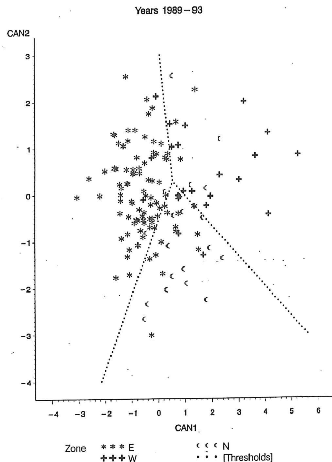
Figure 1 Distribution of the observations in the space of the canonical variates (CAN1 and CAN2). Observations from the Eastern, Northern and Western zones of Tuscany are labeled «E», «N» and «W» respectively. The dotted lines correspond to the between-zone threshold. These are derived from the linear discriminant function including the two canonical variates.
