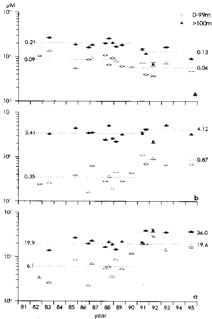
Figure 1. Mean concentrations of \text{P-PO}_4 (a), \text{N-(NO}_2 + \text{NO}_3) (b) and mean \text{N:P} values (c) in all the cruises carried out in the Northern Tyrrhenian Sea and in the two layers. General means for the periods 1982–1990 and 1991–1995 are indicated.
