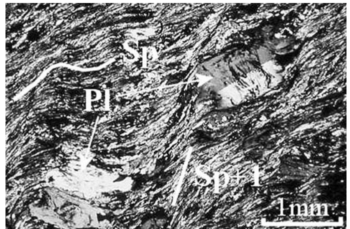
Fig. 2 - b) Plagioclase porphyroblasts (Pl) enveloped by Sp, crossed polars, micaschist, well Selvaccia 3, 2620 m, Larderello field.
