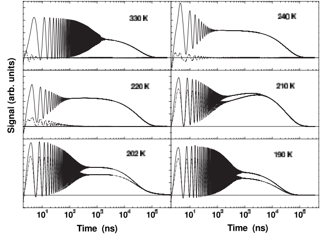
FIG. 2. VV (—) and HH (···) signals at six different temperatures. For the three highest temperatures, the dots (···) do not represent the HH signal but the difference between the VV and HH signals.
