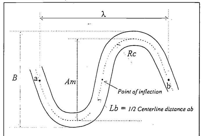
Figure 2. Sketch of Idealized Meander (Leopold & Wolman, 1960, modified).
