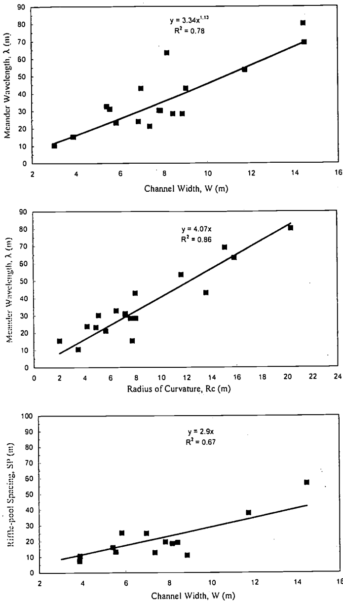
Figure 3. Regression Equations for Maryland Streams.
