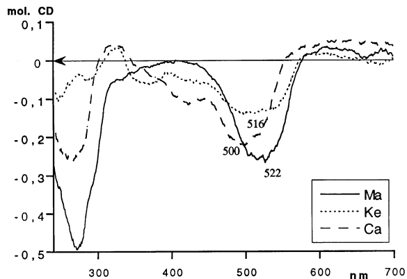
Fig. 7. CD spectra of Ma, Ke and Ca ( 1.18 \times 10^{-4} M), recorded within few minutes after dissolution.
