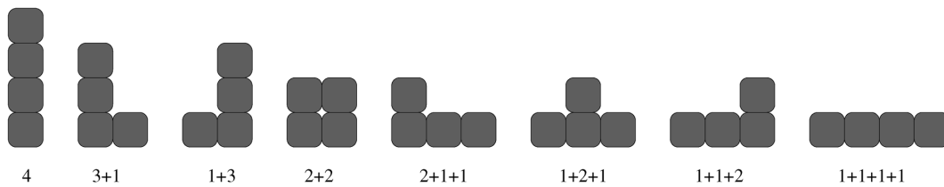
Figure 1.1: Bargraphs associated to compositions of number 4
