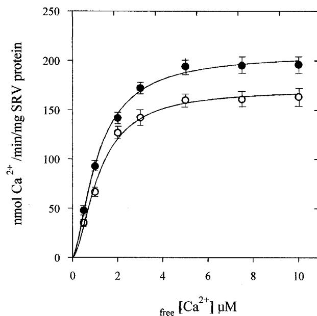
FIG. 10. \text{Ca}^{2+} uptake of PKA phosphorylated SRVs as a function of free \text{Ca}^{2+} concentration. SRVs were phosphorylated as described under "Materials and Methods," and aliquots were taken and assayed for \text{Ca}^{2+} uptake in the standard reaction medium in the absence (○) and in the presence (●) of 100 units of acylphosphatase. Each point represents the mean value \pm S.E. of five determinations.
