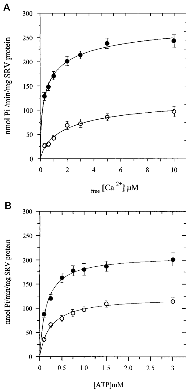
FIG. 6. Cardiac SR Ca 2+ ATPase activity as a function of free Ca 2+ (A) and ATP (B) concentrations. SRVs (50 μg/ml) were assayed in the absence (○) and in the presence (●) of 100 units of acylphosphatase. Each point represents the mean value ± S.E. of five determinations.
