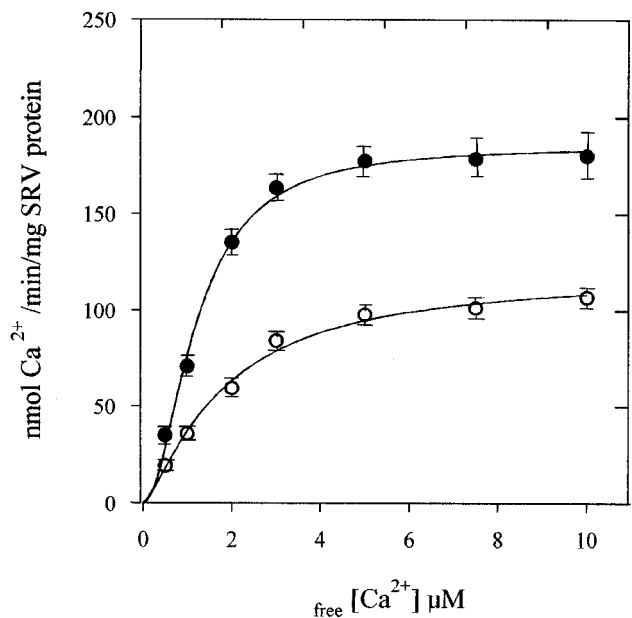
FIG. 7. Cardiac SR Ca 2+ uptake as a function of free Ca 2+ concentration. SRVs (50 μg/ml) were assayed in the absence (○) and in the presence (●) of 100 units of acylphosphatase. Each point represents the mean value ± S.E. of five determinations.
