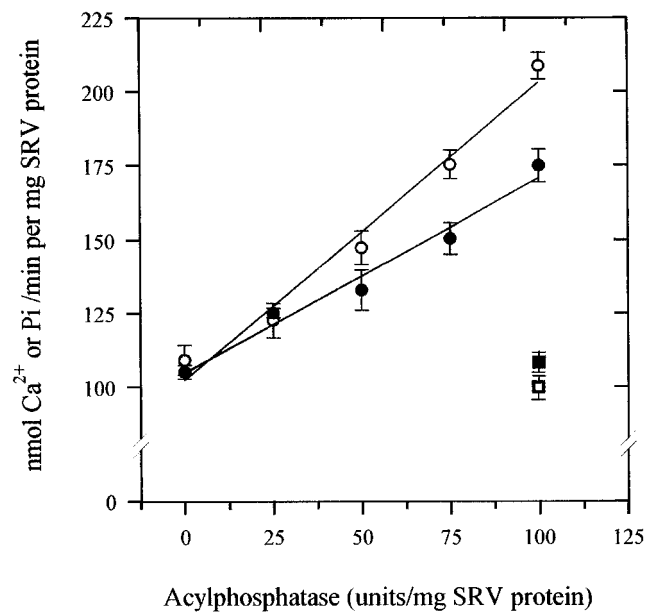
FIG. 5. Effect of different acylphosphatase concentrations on \text{Ca}^{2+} ATPase activity and \text{Ca}^{2+} uptake of cardiac SRVs. \text{Ca}^{2+} ATPase activity (○) and \text{Ca}^{2+} uptake (●) were assayed as described under "Materials and Methods." \text{Ca}^{2+} -ATPase activity was expressed as nmol of ATP split per min/mg of SRV protein and \text{Ca}^{2+} uptake as nmol of \text{Ca}^{2+} transported into vesicles per min/mg of SRV protein. Each point represents the mean value \pm S.E. of five determinations. Changes observed in \text{Ca}^{2+} -ATPase activity and \text{Ca}^{2+} transport, with increasing amounts of acylphosphatase, were statistically significant ( p < 0.01 by the one way analysis of variance). □ and ■, respectively, indicate the values obtained for \text{Ca}^{2+} ATPase activity and \text{Ca}^{2+} uptake with an amount of heat-denatured acylphosphatase corresponding to 100 units of the active enzyme.
