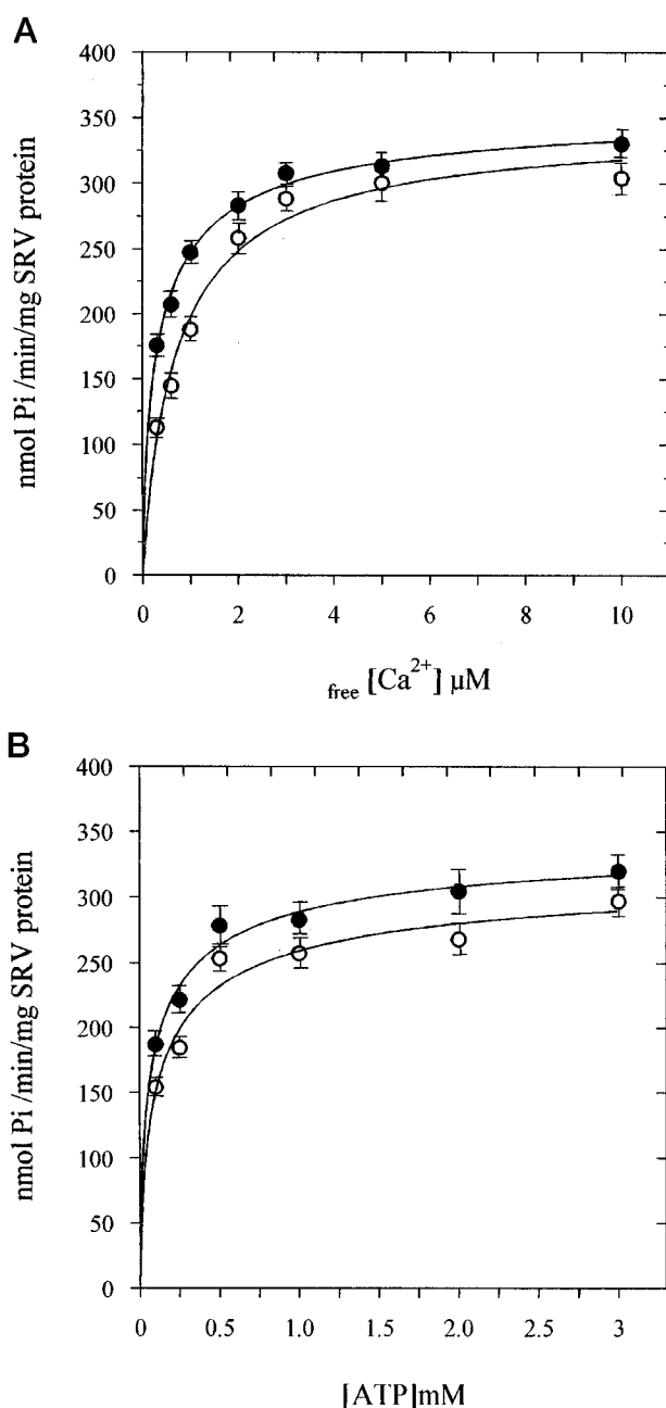
FIG. 9. \text{Ca}^{2+} ATPase activity of PKA-phosphorylated SRVs as a function of free \text{Ca}^{2+} (A) and ATP (B) concentrations. SRVs were phosphorylated as described under "Materials and Methods," and aliquots were taken and assayed for \text{Ca}^{2+} ATPase activity in the standard reaction medium in the absence (○) and in the presence (●) of 100 units of acylphosphatase. Each point represents the mean value \pm S.E. of five determinations.
