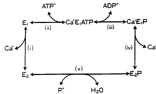
FIG. 11. A scheme of \text{Ca}^{2+} pump ATPase. The scheme is based on that reported by Tada et al. (3). E 1 and E 2 represent two different forms of the enzyme, which exhibit higher and lower affinities for \text{Ca}^{2+} , respectively; i and o indicate the inside and outside of SR membranes. E 1 P is the form of the phosphorylated intermediate having higher affinity for \text{Ca}^{2+} , while E 2 P has a lower affinity for \text{Ca}^{2+} .
