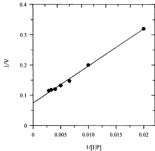
FIG. 2. Initial rate of acylphosphatase-induced dephosphorylation of cardiac SR \text{Ca}^{2+} -ATPase phosphoenzyme as a function of EP concentration. 100 units of acylphosphatase were incubated in 30 mM Tris-HCl, pH 7.4, at 37 °C with differing amounts of labeled vesicles. EP concentration [EP] was expressed as pmol of ^{32}\text{P} bound per ml. The initial rate of dephosphorylation (V), net for spontaneous hydrolysis, was expressed as pmol of ^{32}\text{P} released per min/ml. Each point represents the mean value of five determinations. Data are shown as a double reciprocal plot.
