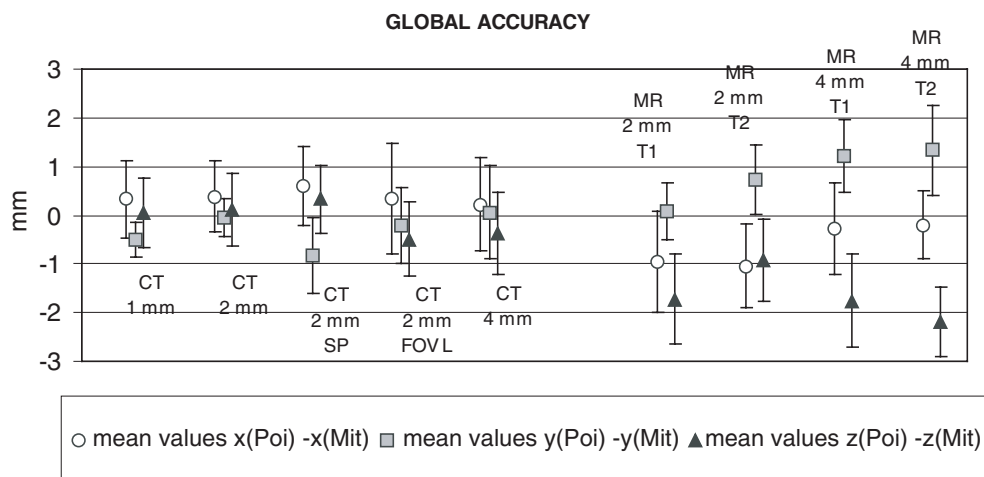
Figure 8. Mean values \overline{\Delta x^{P-M}} , \overline{\Delta y^{P-M}} , \overline{\Delta z^{P-M}} ; \sigma_x^{P-M} , \sigma_y^{P-M} , \sigma_z^{P-M} are shown as error bars. Mean values of procedures based on MR imaging show meaningful deviations from the expected 0 value, especially in the z direction.
