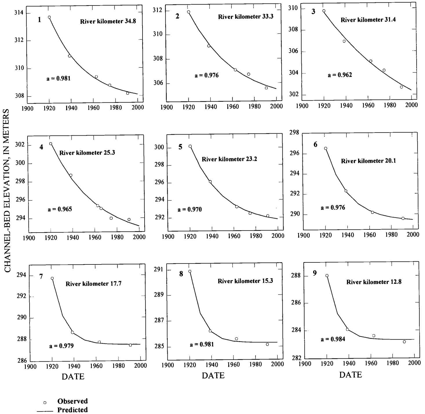
Figure 7. Trends of Degradation at Nine Sites on West Tarkio Creek Fit With Equation (4).
