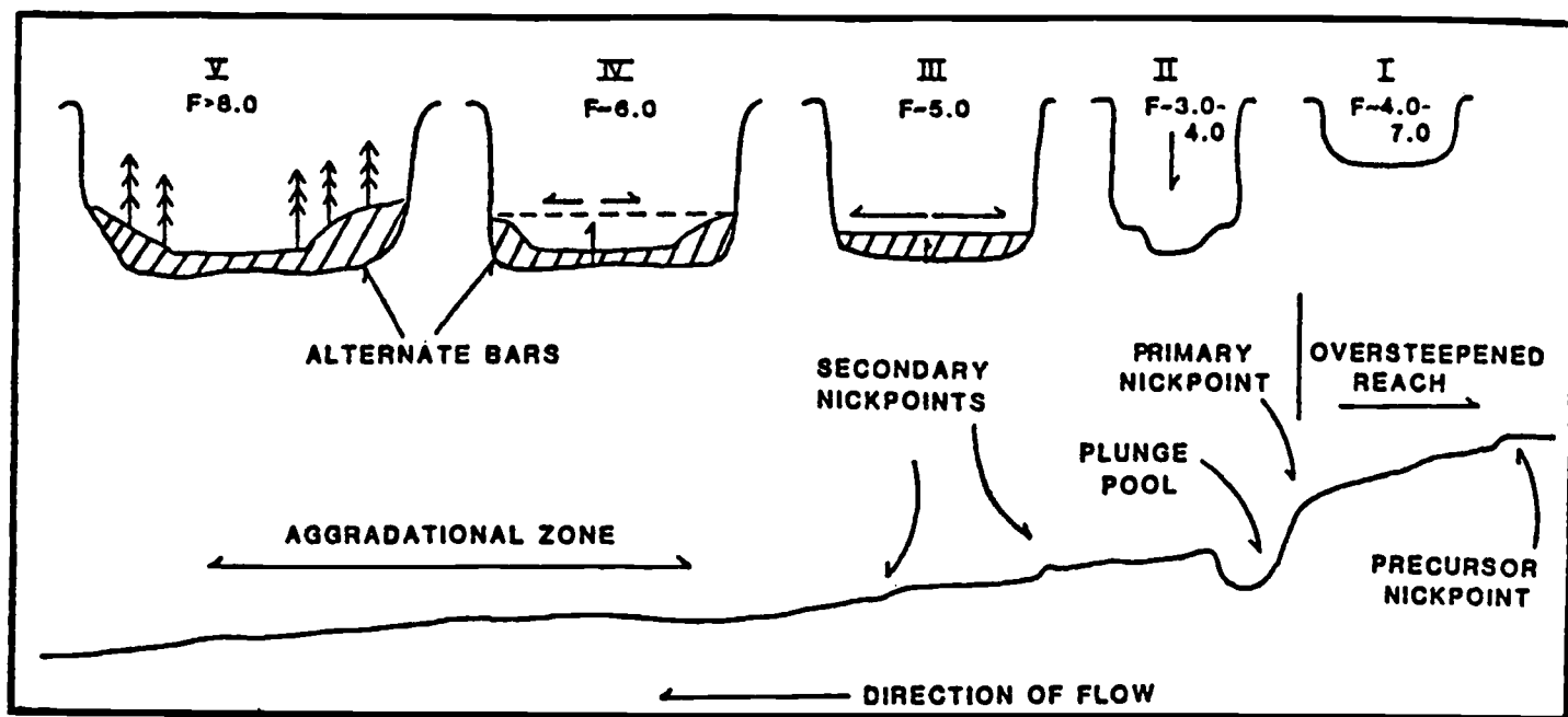
Figure 3. Five-Stage Model of Channel Evolution Developed on Oaklimer Creek, Northern Mississippi (from Schumm et al. , 1984).
