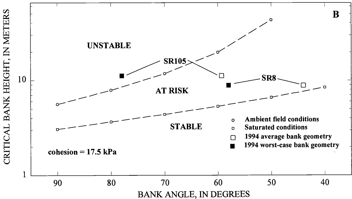
Figure 10. Bank-Stability Chart for Shear-Strength Conditions in the (A) Vicinity of the J52 Bridge Over West Tarkio Creek, Page County, Iowa; Also Used as Representative of Other West Tarkio Creek Sites and (B) Bank-Stability Chart in the Vicinity of the State Route 105 Bridge Over South Fork Big Nemaha River, Southeastern Nebraska; Also Used as Representative of Site at State Route 8.
