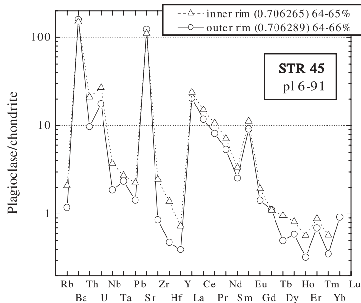
Fig. 9. Chondrite-normalized (Anders & Grevesse, 1989) trace element patterns for a plagioclase of sample STR45. See Fig. 8 for explanation of the element order. Sr isotope ratios and anorthite content (%) of the analysed zones are also given in the legend.
