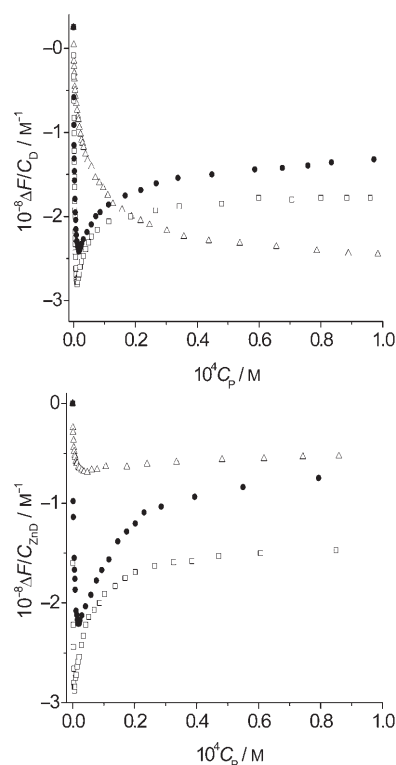
Figure 4. Top: Binding isotherms in fluorescence detection for the D –DNA system at different ionic strengths. \square : I=0.01 M; \bullet : I=0.11 M; \triangle : I=1.01 M. \lambda_{\text{em}}=500 nm, pH 7.0, 298.1 K. Bottom: Binding isotherms in fluorescence detection for the [Zn D ]-DNA system at different ionic strengths. \square : I=0.01 M; \bullet : I=0.11 M; \triangle : I=1.01 M. \lambda_{\text{em}}=500 nm, pH 8.0, 298.1 K. C_{\text{D}}=C_{[\text{ZnD}]}=1 \times 10^{-6} M.
