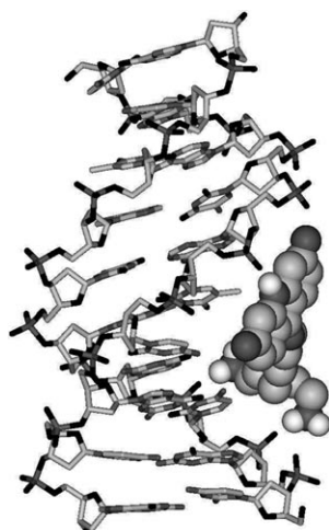
Figure 10. Adduct obtained with the CGCGATATCG sequence featured by major-groove-binding mode. \Delta E is calculated interaction energy.
