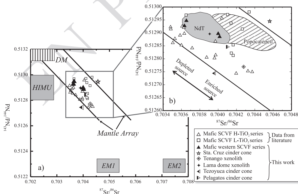
Figure 10. ^{143}\text{Nd}/^{144}\text{Nd} vs. ^{87}\text{Sr}/^{86}\text{Sr} for mafic volcanic rocks ( \text{MgO} \geq 6.0 wt.%), Sta Cruz cinder cone and crustal xenoliths of the Tenango area. a) DM: Depleted mantle; EM1: enriched mantle 1; EM2: enriched mantle 2; HIMU: high ^{238}\text{U}/^{204}\text{Pb} mantle; data from Zindler and Hart (1986). b) The gray-filled area represents the isotopic ratios of nearby Nevado de Toluca volcano (NdT), whereas the area filled with the line pattern represents data from Popocatepetl volcano. Data provenance: Verma (2000); Velasco-Tapia (2002); Martínez-Serrano et al. , 2004, Siebe et al. (2004b) and Schaaf et al. (2005).
