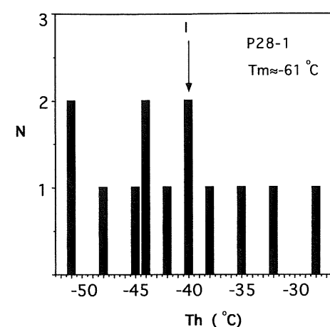
Fig. 7. Microthermometry histogram of the trail of secondary inclusions P28-1. Roman number refers to the inclusions selected for RAMAN analysis. Th = homogenization temperature L-V(L), Tm = final melting temperature of CO 2 . Total N = 13.
