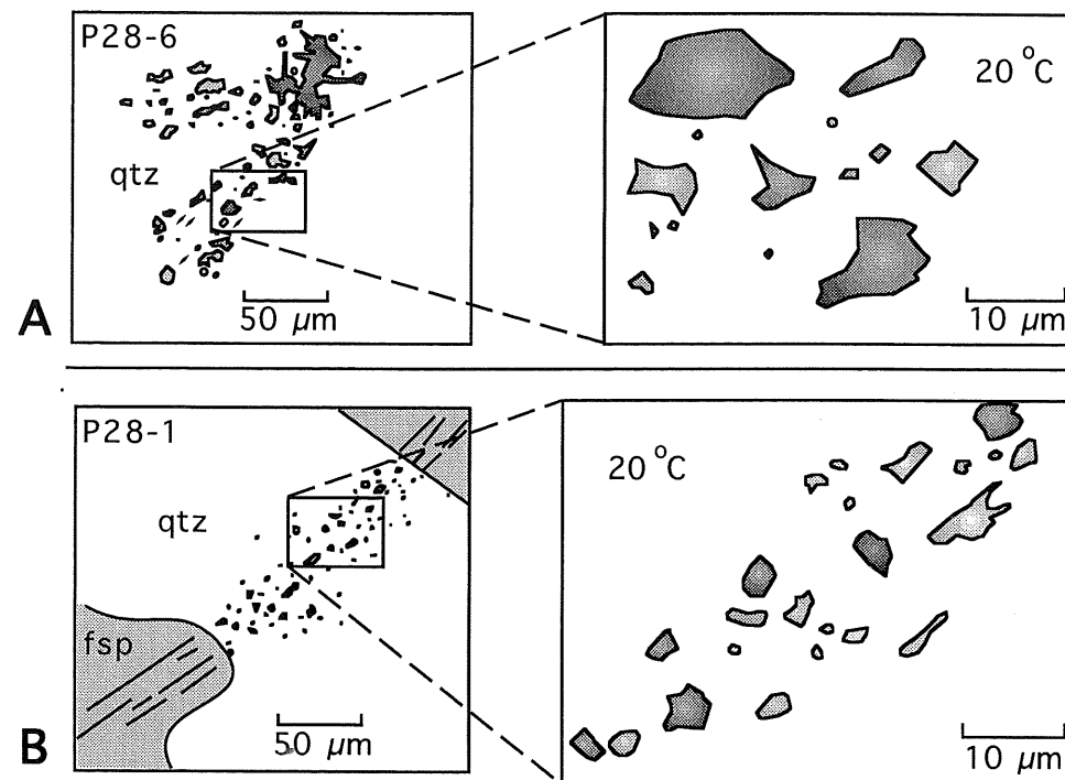
Fig. 5. Sketches of A) primary (P28-6) and B) secondary (P28-1) inclusions at room temperature. A) The exploded primary inclusion is visible in the upper part of the left diagram and is surrounded by the randomly oriented daughter inclusions. B) The secondary inclusions in quartz lie on a trail which crosses mineral boundaries.
