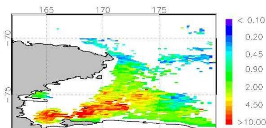
Fig. 3. Satellite Chl-a concentration in the western Ross Sea [SeaWiFS, December 19 to 26, 1997]. The color code refers to concentrations in \text{mg}/\text{m}^3 .
