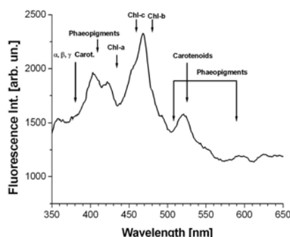
Fig. 4. Excitation spectra at the hydrographic station 4 of Table 1 [ \lambda_{\text{em}}=680 \text{ nm} ].
