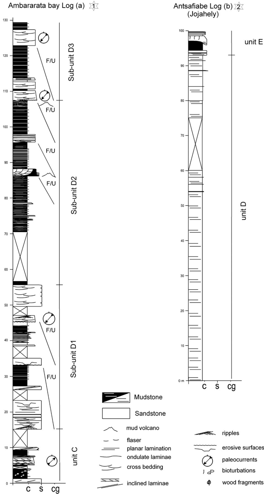
Fig. 4. (a) Ambarata Bay section: This succession is referred to a fluvial–floodplain setting characterized by cyclic change of the depositional environment such as channels, floodplain and ponds. (b) Antsafiabe section: The fine-grained deposits observed in this section document a fluvial low-energy, depositional environment under a different hydrological regime compared to the muddy deposits within unit D in the Ambarata Bay.
