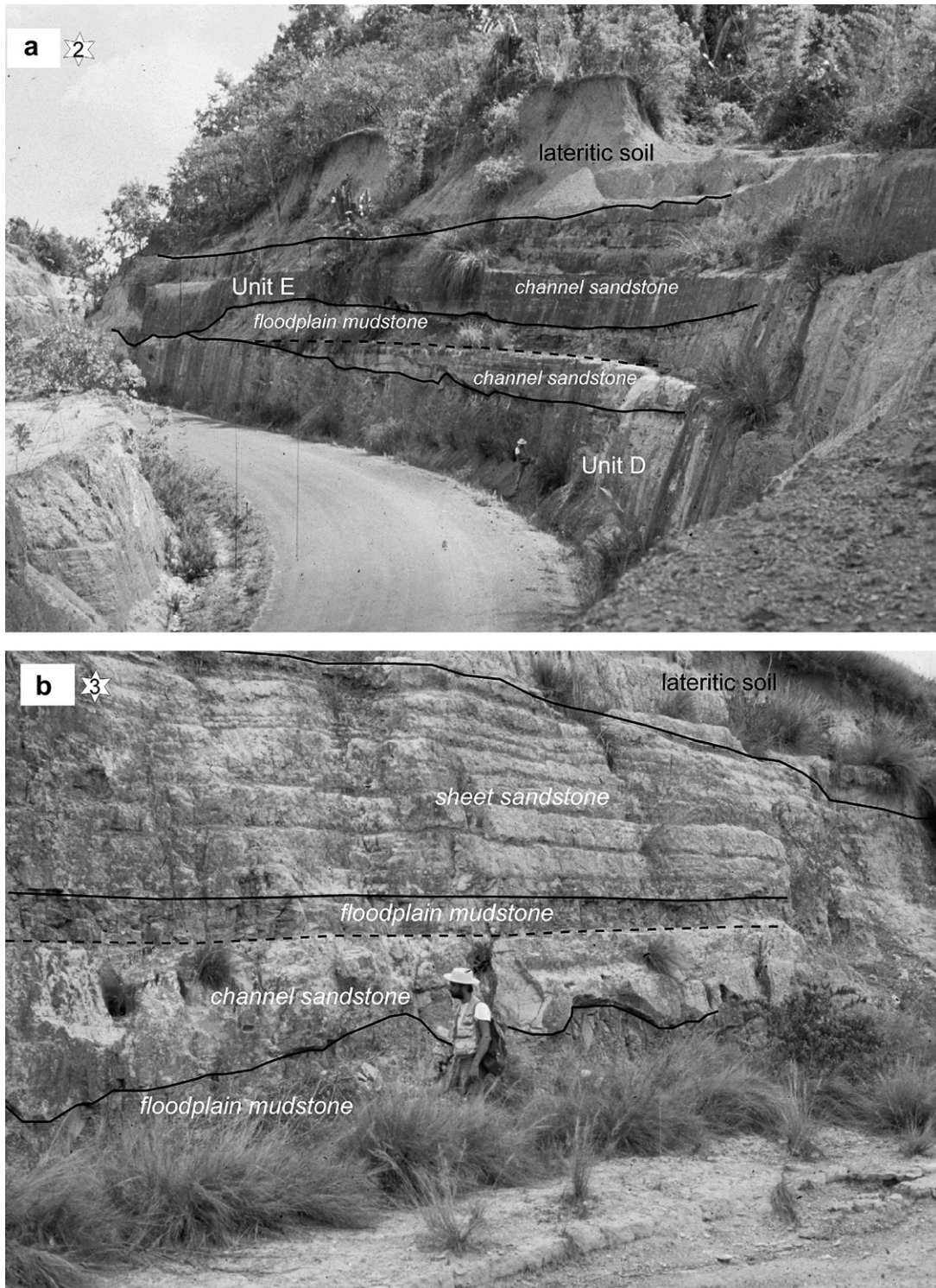
Fig. 6. (a) The upper portion of Antsaftabe section shows the transition from unit D to unit E, person for scale; (b) unit E at Ankarami characterized by channellized sandstone passing upward into sheet sandstones, person for scale.
