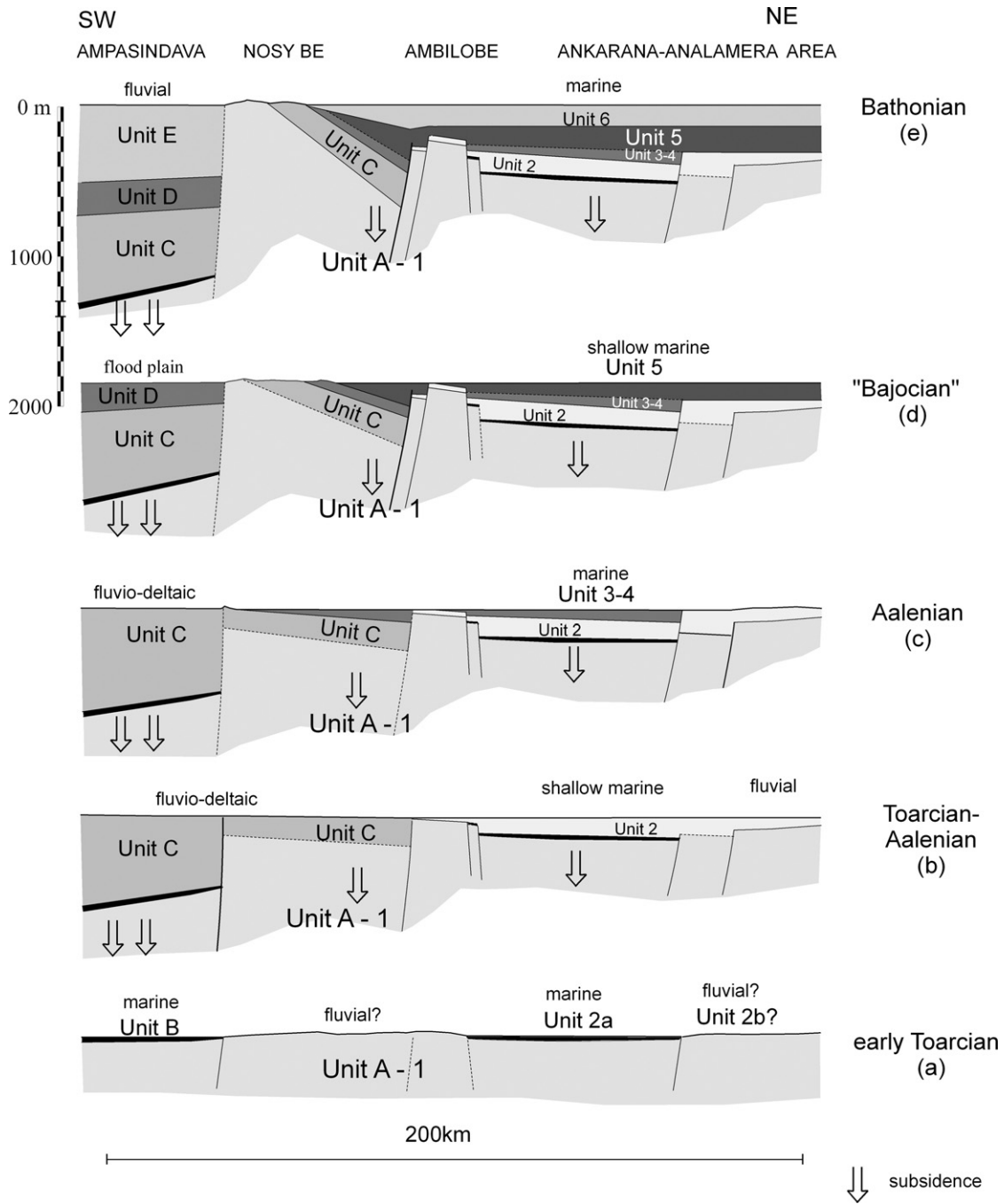
Fig. 10. Tectono-sedimentary cross-sections of the Antsiranana Basin from the Toarcian to Bathonian illustrate Early Toarcian: widespread marine transgression over the Isalo Sandstones. Late Toarcian–early Aalenian: the basin underwent significant depositional differentiation with activation of asymmetric sub-basins bounded by steep faults. Aalenian: more pronounced subsidence and block tilting in the central-southwestern part of the Ankarana–Analamera. Bajocian–Bathonian: the Nosy Be high was a major structural element in the basin separating differently subsiding zones.
