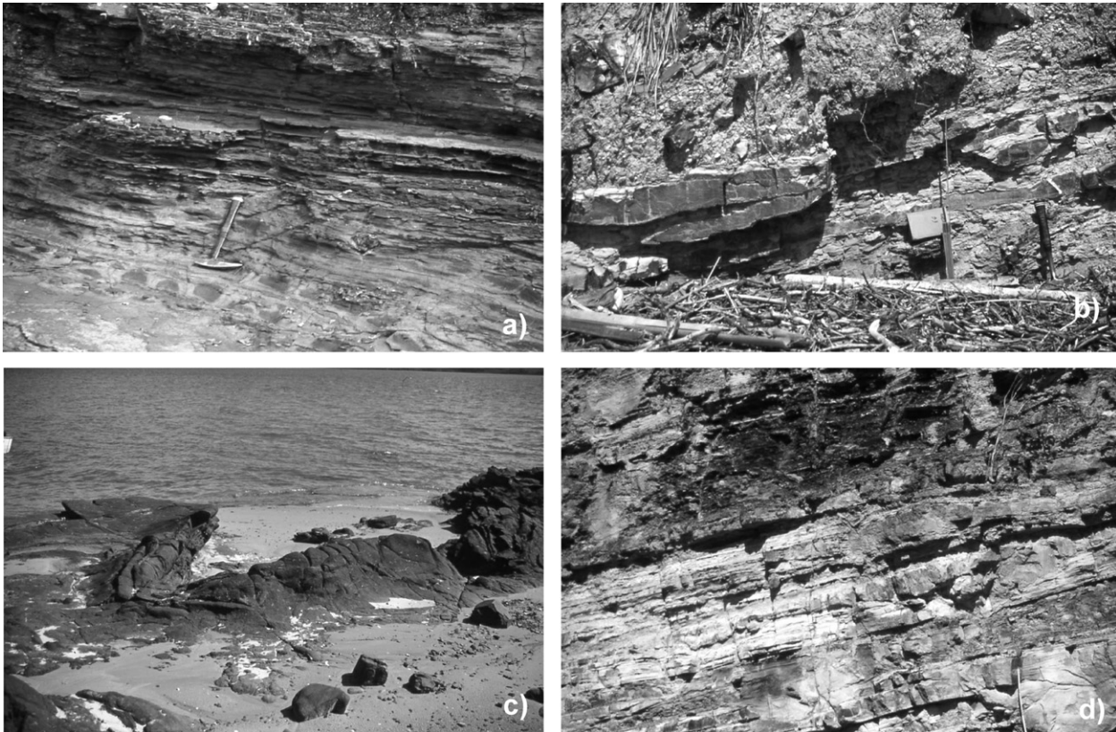
Fig. 5. (a) Thinly stratified black calcilutites of unit C exposed on the bank of the Bemanevika estuary, hammer for scale (see Table 1); (b) channellized sandstones and interbedded mudstone of sub-unit D1 in the Ambarata Bay area, hammer for scale (see also Fig. 5a); (c) large-scale mud volcano affects a 1.5 m thick calcarenite bed which is overlain by undisturbed laminated mudstones, sub-unit D2, Ambarata Bay; (d) sheet sandstone and interbedded mudstone in sub-unit D3, Ambarata Bay, the rod is 1 m long.
