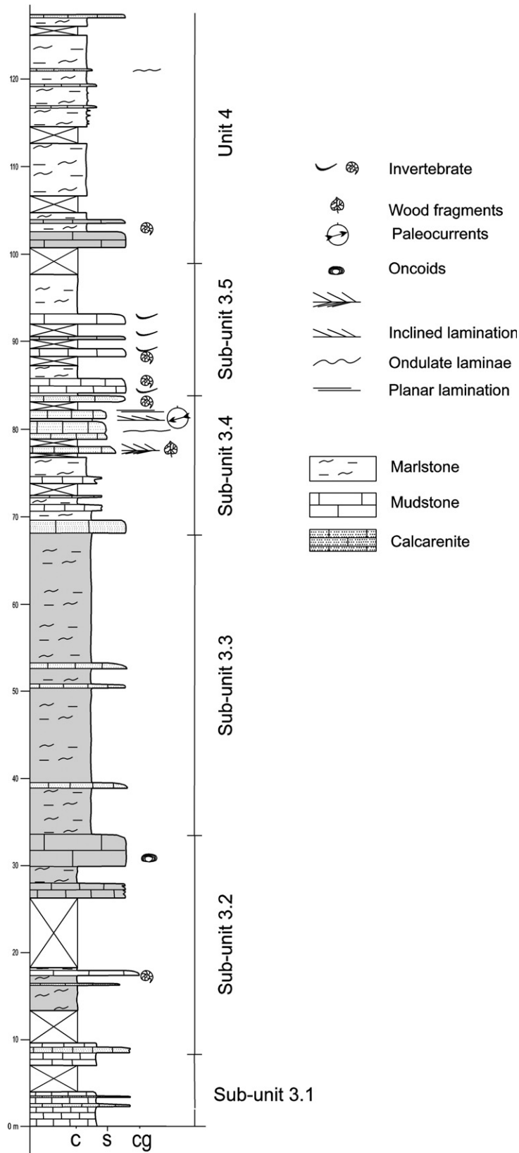
Fig. 8. (a) Anivorano section; (b) panoramic view of the Ampatsoa ridge and interpretative line-drawing showing the stratigraphic transition between units 4 and 5 and the internal stacking of exposed intervals within unit 5 discussed in the text; (c) Ankarabo section. The units 3 and 4 show a cyclic facies development which is interpreted in terms of relative sea level fluctuations affecting a mixed carbonate–siliciclastic ramp during part of the Aalenian. The unit 5 is interpreted as a carbonate platform with the deposition of carbonate mud in a lagoonal environment and the deposition of ooid shoals and in barriers at the platform rim.
