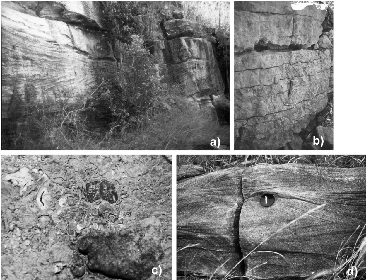
Fig. 9. (a) Planar cross-stratified sandstone of sub-unit 2a exposed in the Ankarabo area (see Table 2); (b) Anivorano section: detail on the mudstones on top of sub-unit 3.2 showing a thickening-upward trend, hammer for scale; (c) oncolitic limestone of interval 5.4a exposed in the Ampatsoa Ridge (Fig. 7b); (d) hummocky cross stratification in the oolitic grainstone of the interval 5.5a exposed in the Ampatsoa Ridge, cap lens for scale.
