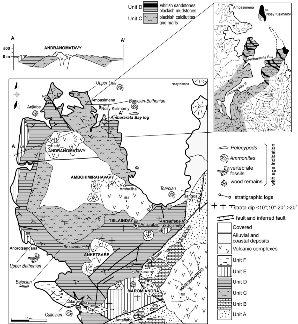
Fig. 3. Geological map of the Ampasindava Peninsula; inset with distribution of units C and D in the Ambarata Bay–Bemanevika estuary area.
