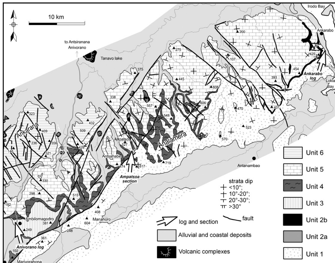
Fig. 7. Geological map of the Ankarana–Analamera region showing the relations among the Lower–Middle Jurassic units defined in this study.
