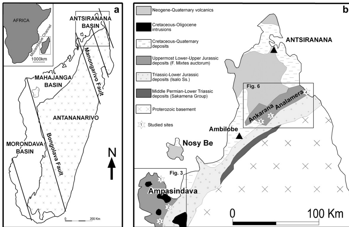
Fig. 1. (a) Distribution of the main sedimentary basins and fault zones in Madagascar; to notice the NW–SE trending major fault zones; (b) schematic geological map of the Antsiranana Basin.
