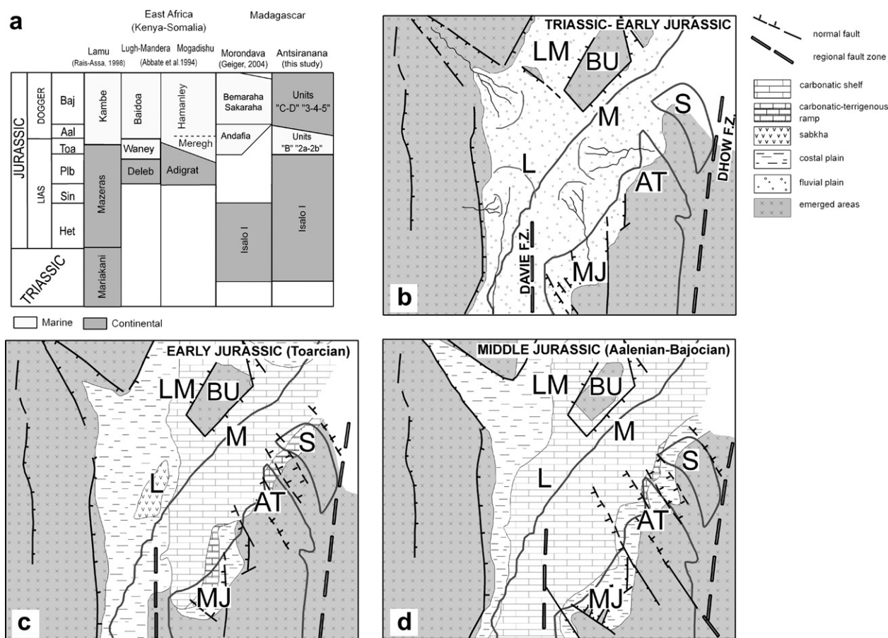
Fig. 11. (a) comparative stratigraphy of the Triassic–Middle Jurassic successions of East Africa and NW Madagascar–Seichelles (see text for references); (b–d) regional paleogeographic maps discussed in the text. Codes for the basins (see text for details): LM, Lugh-Mandera; M, Mogadishu; L, Lamu; S, Seichelles; AT, Antsiranana; MJ, Mahajanga.
