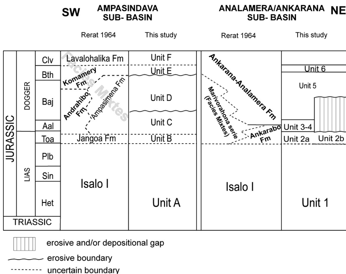
Fig. 2. Comparison of the stratigraphic subdivisions of the Lower–Middle Jurassic successions in the Antsiranana Basin. This succession rests unconformably on Middle Permian to Lower Jurassic Karoo deposits (Sakamena and Isalo groups, and started to develop during the Early–Middle Toarcian when shallow marine conditions established over the basin bringing to the deposition of mixed carbonate–terrigenous deposits.
