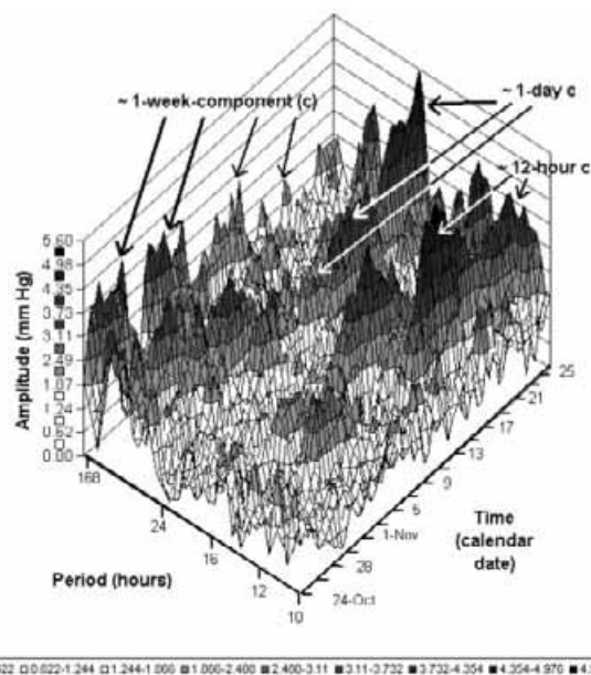
Figure 28 Changing amplitude of some components in a partial spectral element of the postnatal human diastolic blood pressure chronome. Data from a healthy boy, born 19.10.1992, whose blood pressure was measured at mostly 30-minute intervals from 20.10 for the ensuing 40 days, and analyzed as a moving spectrum in separate weekly intervals, displaced in 12-hour increments through the data set. An initially greater prominence of infradians (see ~1 week c, left), shown by height and shading, corresponding to a larger amplitude, contrasts with the prominence of circadians and circasemidians in later weeks of life, while any ultradians with still higher frequencies and any trends and chaos, two other chronome elements, are here unassessed. Gliding spectral window of amplitudes of diastolic blood pressure, focusing on infradians and circadians (side view) in the first 40 days of life of a boy born at term (FW). The prominence of the infradian spectral components immediately after birth is apparent from shading, height and arrows [165,166]. Original data of Yoshihiko Watanabe.
