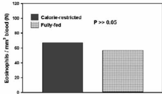
Figure 2 Confusing results one week later: follow-up with more animals starting at an earlier clock hour shows "no difference". A phase difference between the two groups was predicted. The large inter-group difference in eosinophil count was not replicated when more animals were used with an earlier start.
