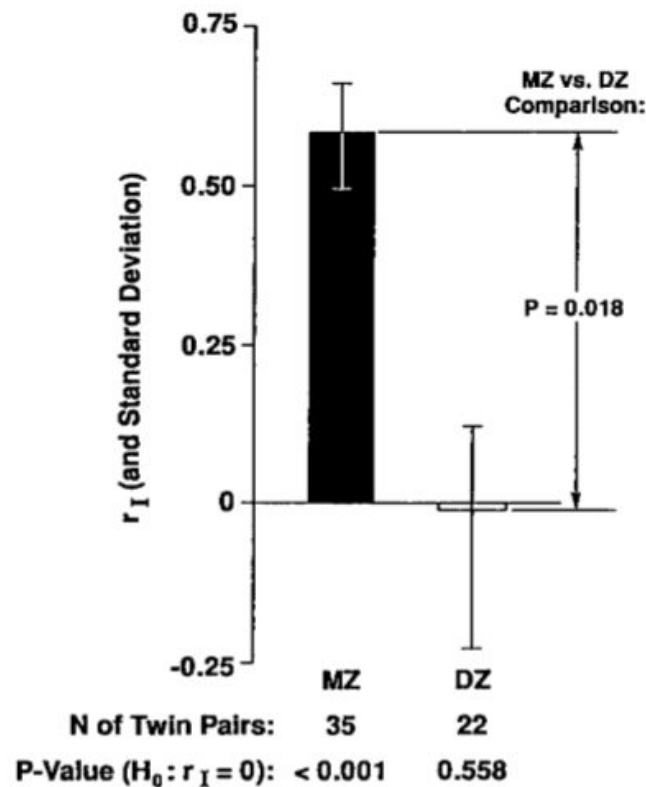
Figure 42 Emergent heritability of the circadian amplitude of human heart rate. Assessed by statistically significant intra-class correlation ( r_I ) for monozygotic (MZ) but not for dizygotic (DZ) twin pairs reared apart. Heart rate was assessed in 24-hour electrocardiograms, amplitude was computed by cosinor; a statistically significant intra-class correlation ( r_I ) for monozygotic (MZ) but not for dizygotic (DZ) twin pairs reared apart was found [85,304].
