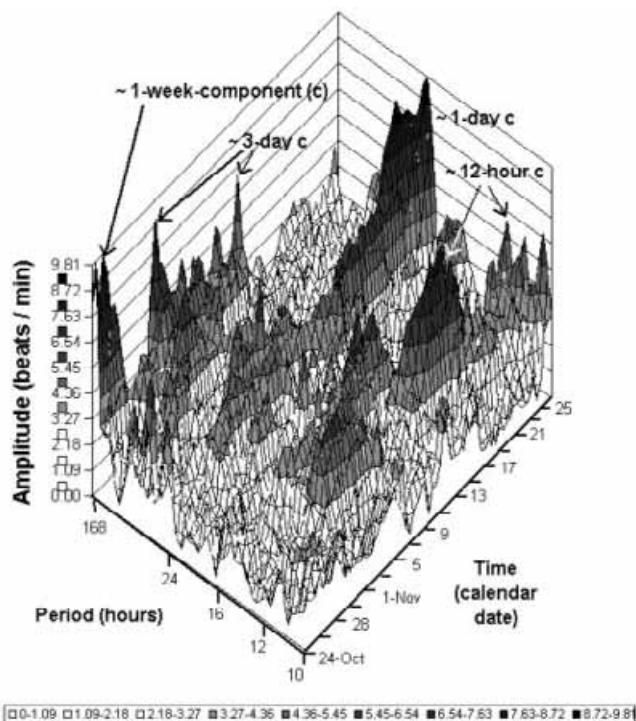
Figure 30 Changing amplitude of some components in a partial spectral element of the postnatal human heart rate chronome. Data from a healthy boy, born 19.10.1992, whose heart rate was measured at mostly 30-minute intervals from 20.10 for the ensuing 40 days, and analyzed as a moving spectrum in separate weekly intervals, displaced in 12-hour increments through the data set. An initially greater prominence of infradians (see ~1 week c, left), shown by height and shading, corresponding to a larger amplitude, contrasts with the prominence of circadians and circasemidians in later weeks of life, while any ultradians with still higher frequencies and any trends and chaos, two other chronome elements, are here unassessed. Gliding spectral window of amplitudes of heart rate, focusing on infradians and circadians (side view) in the first 40 days of life of a boy born at term (FW). Prominence of infradian spectral components immediately after birth is apparent from shading, height and arrows [165,166]. Original data of Yoshihiko Watanabe.
