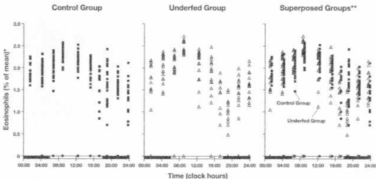
Figure 5 Effect of food restriction on circulating eosinophils in mice. *After \log_{10} -transformation of data expressed as percentage of mean. **To reveal the difficulty to resolve differences by the naked eye alone, and the even greater difficulty of quantifying the patterns of each group and any inter-group differences. There is a need to cover the 24-hour time scale to look for intergroup differences in the face of a large variability, what the active Claude Bernard rightly called the "extreme variability of the internal environment" [264]. Our analysis of variance reveals statistically significant time and group effects and interaction in this time-macroscopic approach, shown elsewhere [303].
